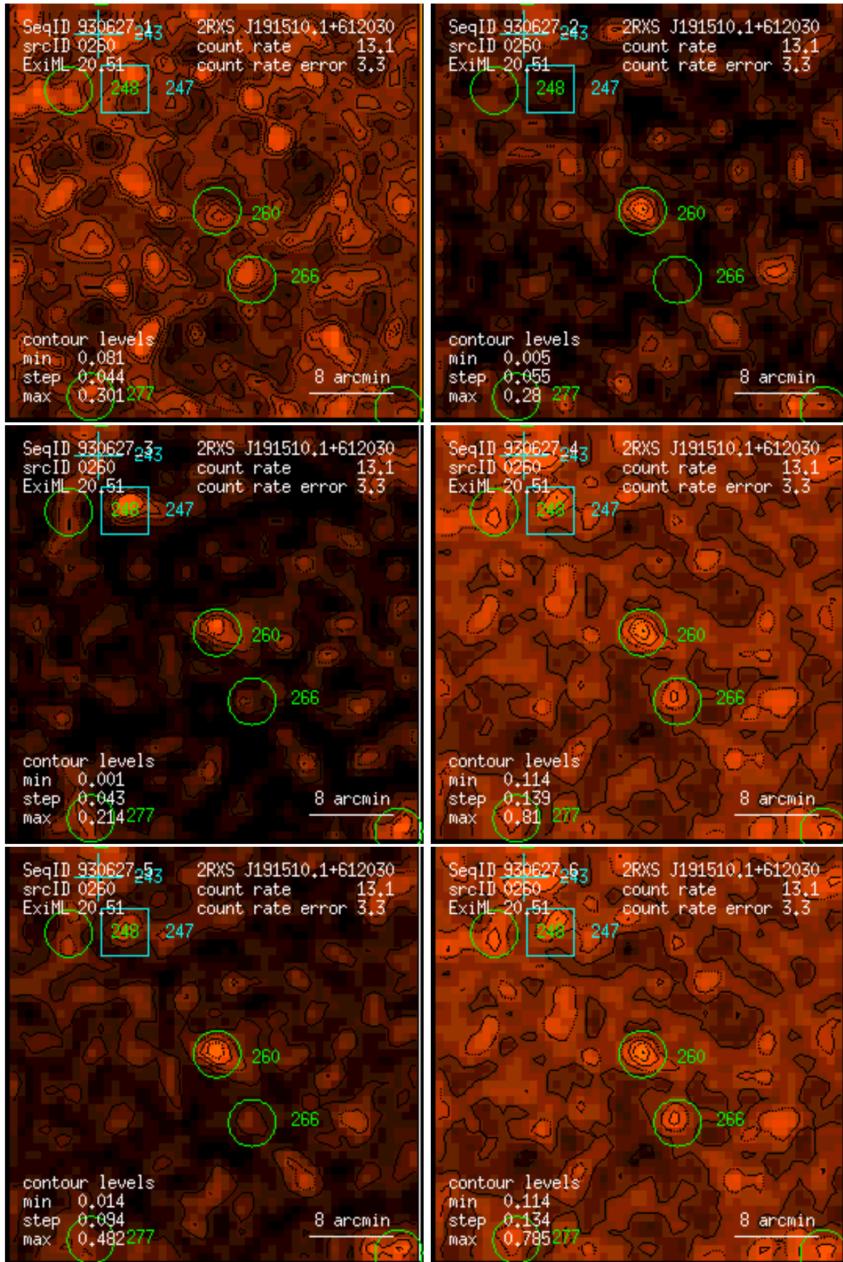
Figure 260: RASS 930627: detection 0260: band rate images, Gaussian filter: (1) PSPC channels 11 – 41, (2) 52 – 90, (3) 91 – 201, (4) 11 – 235, (5) 52 – 201, (6) 11 – 201. Broad band rates in counts/ks. Band rate contour levels in counts/ks/arcmin 2 .
