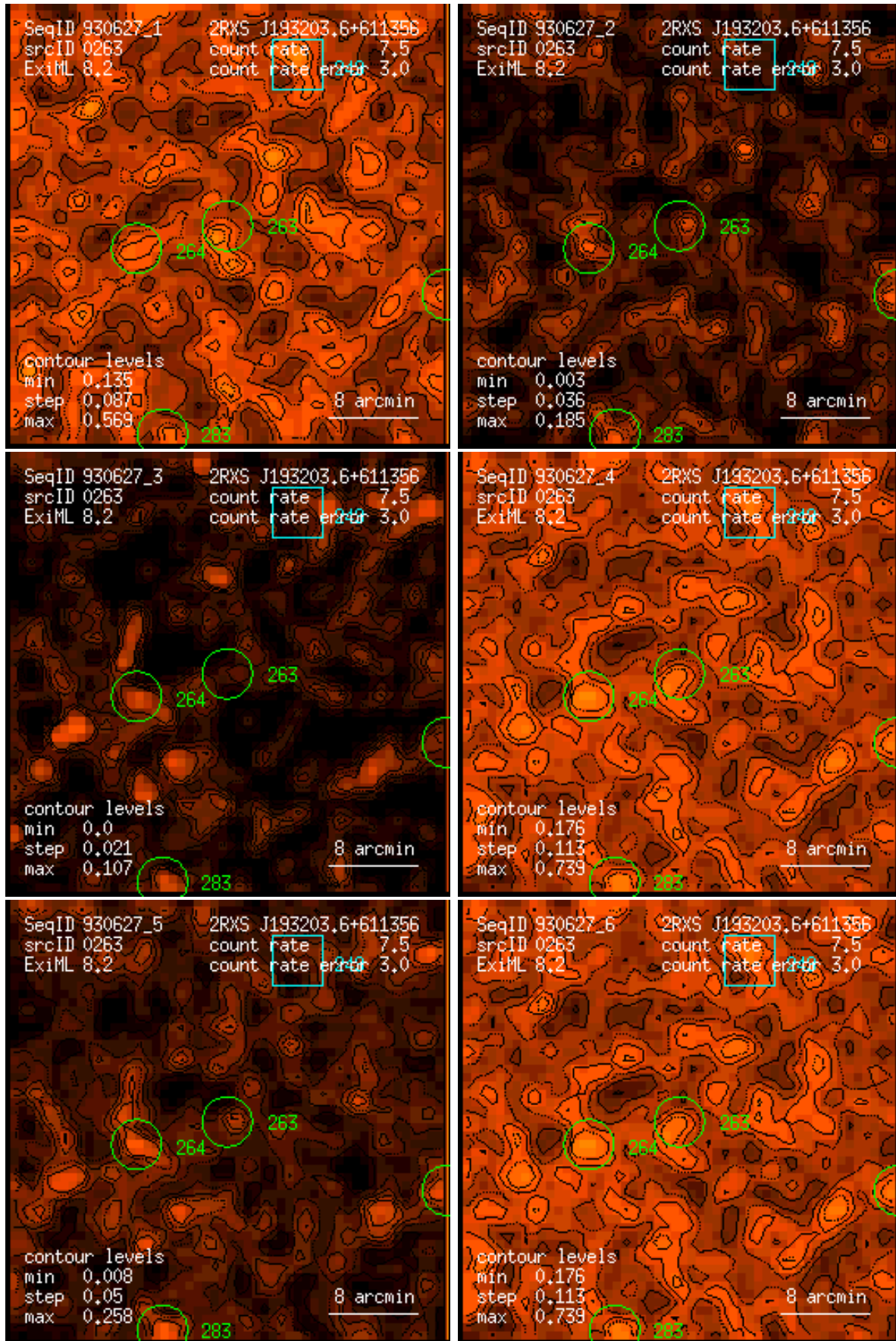
Figure 263: RASS 930627: detection 0263: band rate images, Gaussian filter: (1) PSPC channels 11 – 41, (2) 52 – 90, (3) 91 – 201, (4) 11 – 235, (5) 52 – 201, (6) 11 – 201. Broad band rates in counts/ks. Band rate contour levels in counts/ks/arcmin 2 .
