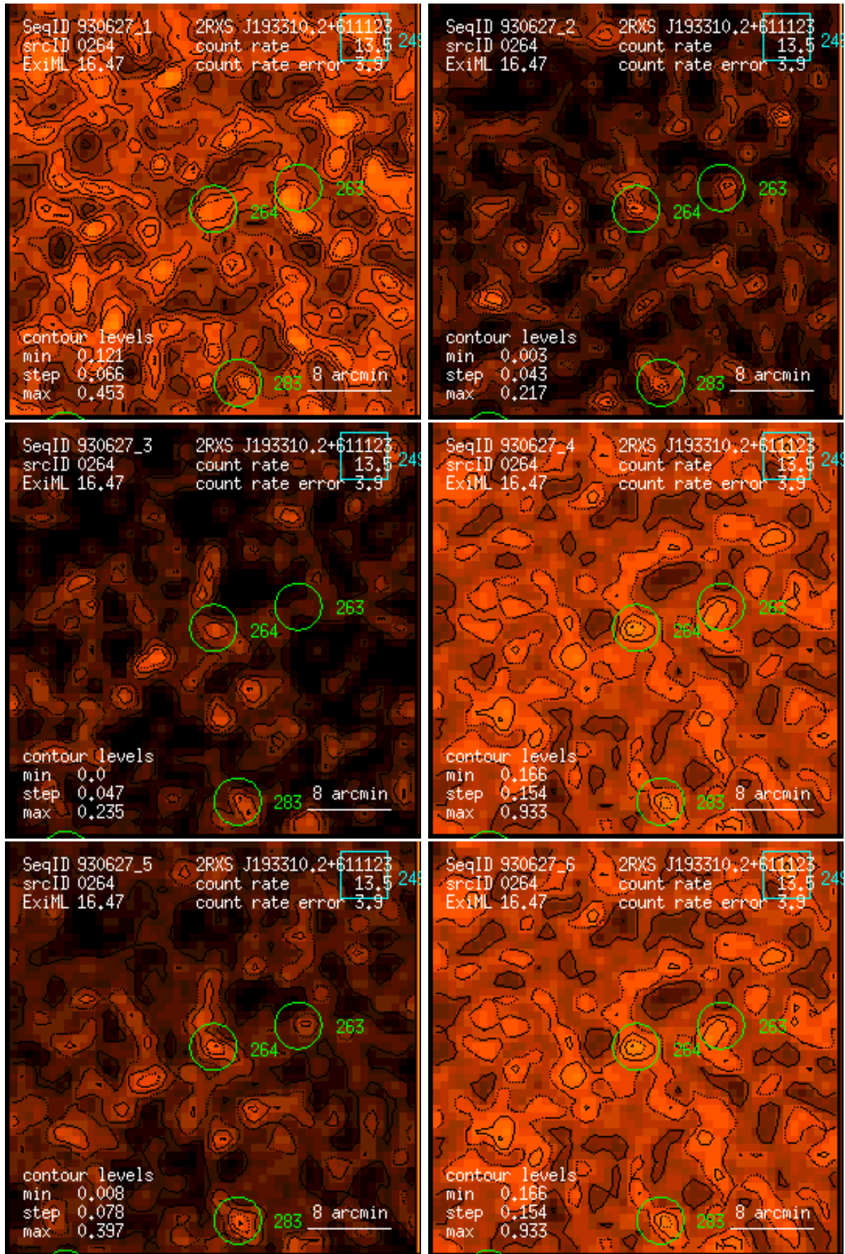
Figure 264: RASS 930627: detection 0264: band rate images, Gaussian filter: (1) PSPC channels 11 – 41, (2) 52 – 90, (3) 91 – 201, (4) 11 – 235, (5) 52 – 201, (6) 11 – 201. Broad band rates in counts/ks. Band rate contour levels in counts/ks/arcmin 2 .
