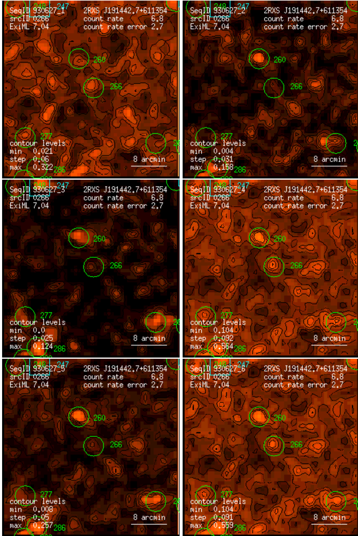
Figure 266: RASS 930627: detection 0266: band rate images, Gaussian filter: (1) PSPC channels 11 – 41, (2) 52 – 90, (3) 91 – 201, (4) 11 – 235, (5) 52 – 201, (6) 11 – 201. Broad band rates in counts/ks. Band rate contour levels in counts/ks/arcmin 2 .
