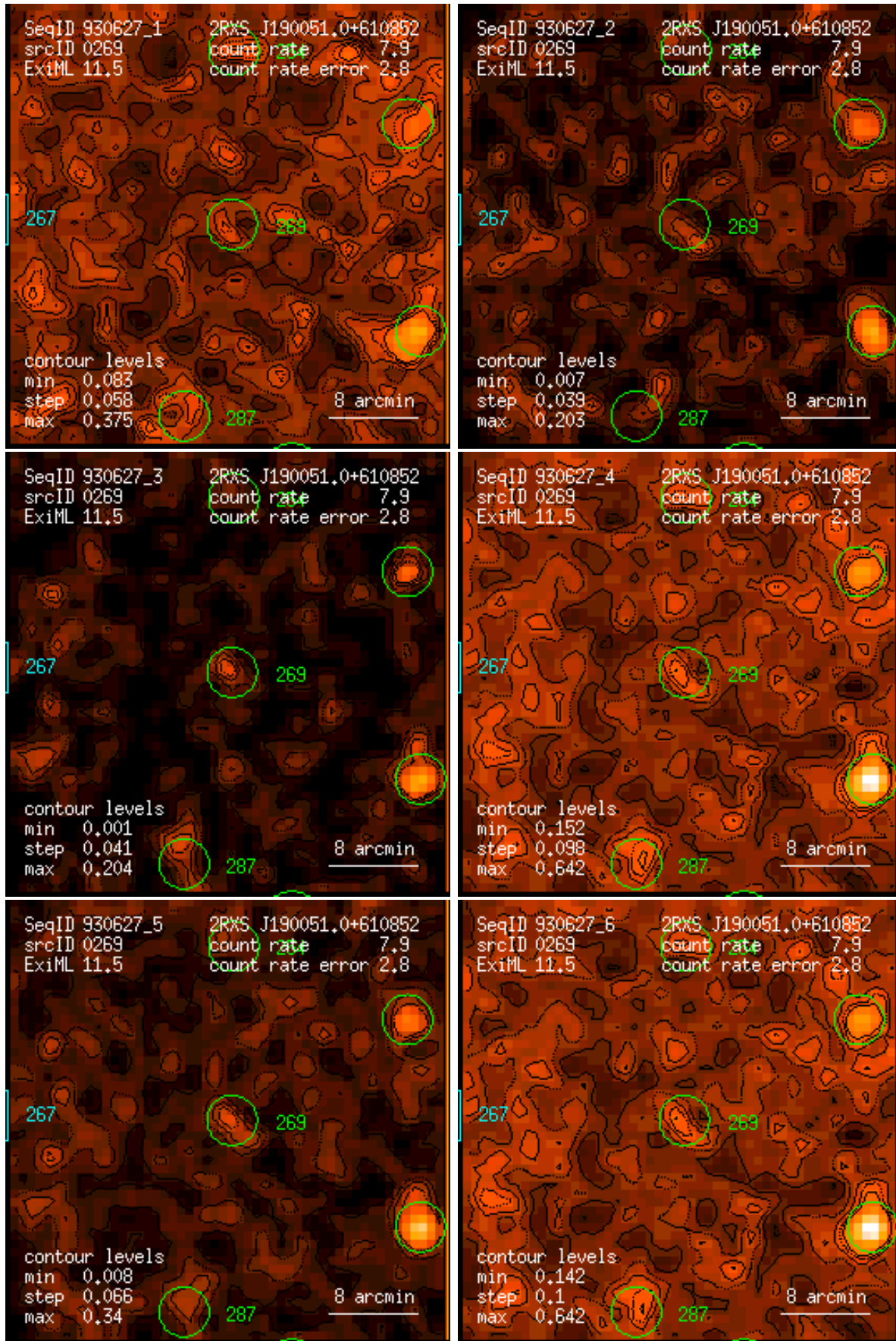
Figure 269: RASS 930627: detection 0269: band rate images, Gaussian filter: (1) PSPC channels 11 – 41, (2) 52 – 90, (3) 91 – 201, (4) 11 – 235, (5) 52 – 201, (6) 11 – 201. Broad band rates in counts/ks. Band rate contour levels in counts/ks/arcmin 2 .
