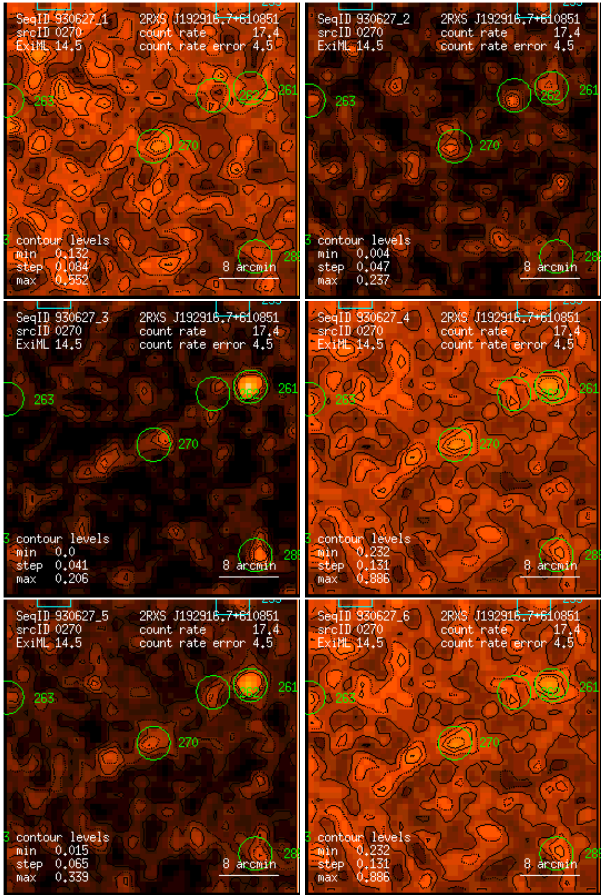
Figure 270: RASS 930627: detection 0270: band rate images, Gaussian filter: (1) PSPC channels 11 – 41, (2) 52 – 90, (3) 91 – 201, (4) 11 – 235, (5) 52 – 201, (6) 11 – 201. Broad band rates in counts/ks. Band rate contour levels in counts/ks/arcmin 2 .
