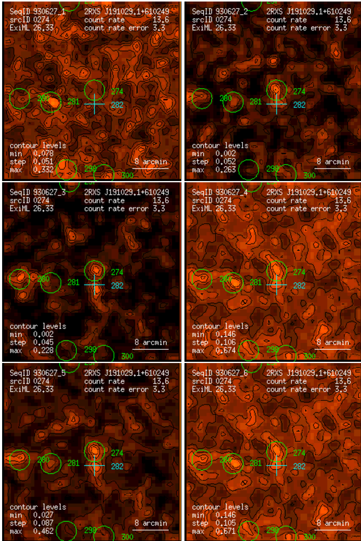
Figure 274: RASS 930627: detection 0274: band rate images, Gaussian filter: (1) PSPC channels 11 – 41, (2) 52 – 90, (3) 91 – 201, (4) 11 – 235, (5) 52 – 201, (6) 11 – 201. Broad band rates in counts/ks. Band rate contour levels in counts/ks/arcmin 2 .
