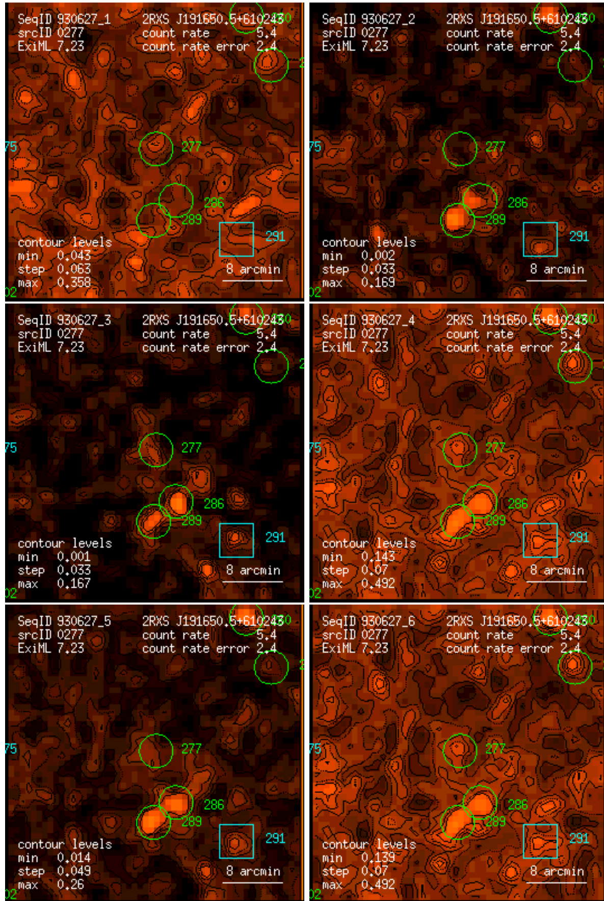
Figure 277: RASS 930627: detection 0277: band rate images, Gaussian filter: (1) PSPC channels 11 – 41, (2) 52 – 90, (3) 91 – 201, (4) 11 – 235, (5) 52 – 201, (6) 11 – 201. Broad band rates in counts/ks. Band rate contour levels in counts/ks/arcmin 2 .
