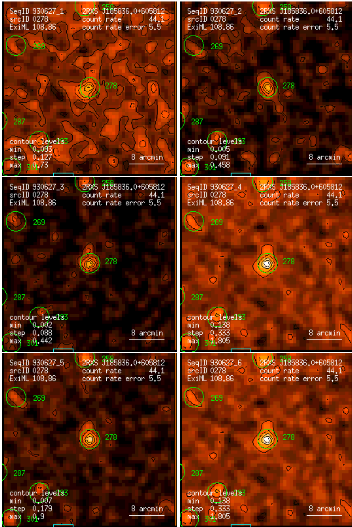
Figure 278: RASS 930627: detection 0278: band rate images, Gaussian filter: (1) PSPC channels 11 – 41, (2) 52 – 90, (3) 91 – 201, (4) 11 – 235, (5) 52 – 201, (6) 11 – 201. Broad band rates in counts/ks. Band rate contour levels in counts/ks/arcmin 2 .
