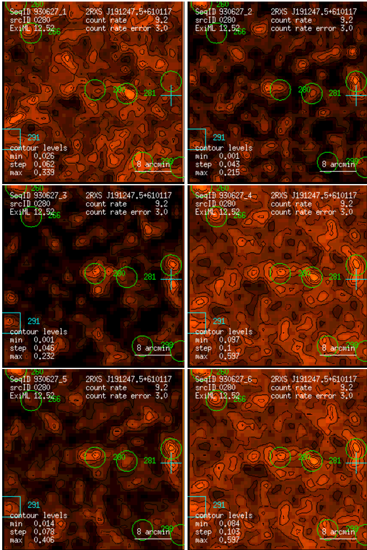
Figure 280: RASS 930627: detection 0280: band rate images, Gaussian filter: (1) PSPC channels 11 – 41, (2) 52 – 90, (3) 91 – 201, (4) 11 – 235, (5) 52 – 201, (6) 11 – 201. Broad band rates in counts/ks. Band rate contour levels in counts/ks/arcmin 2 .
