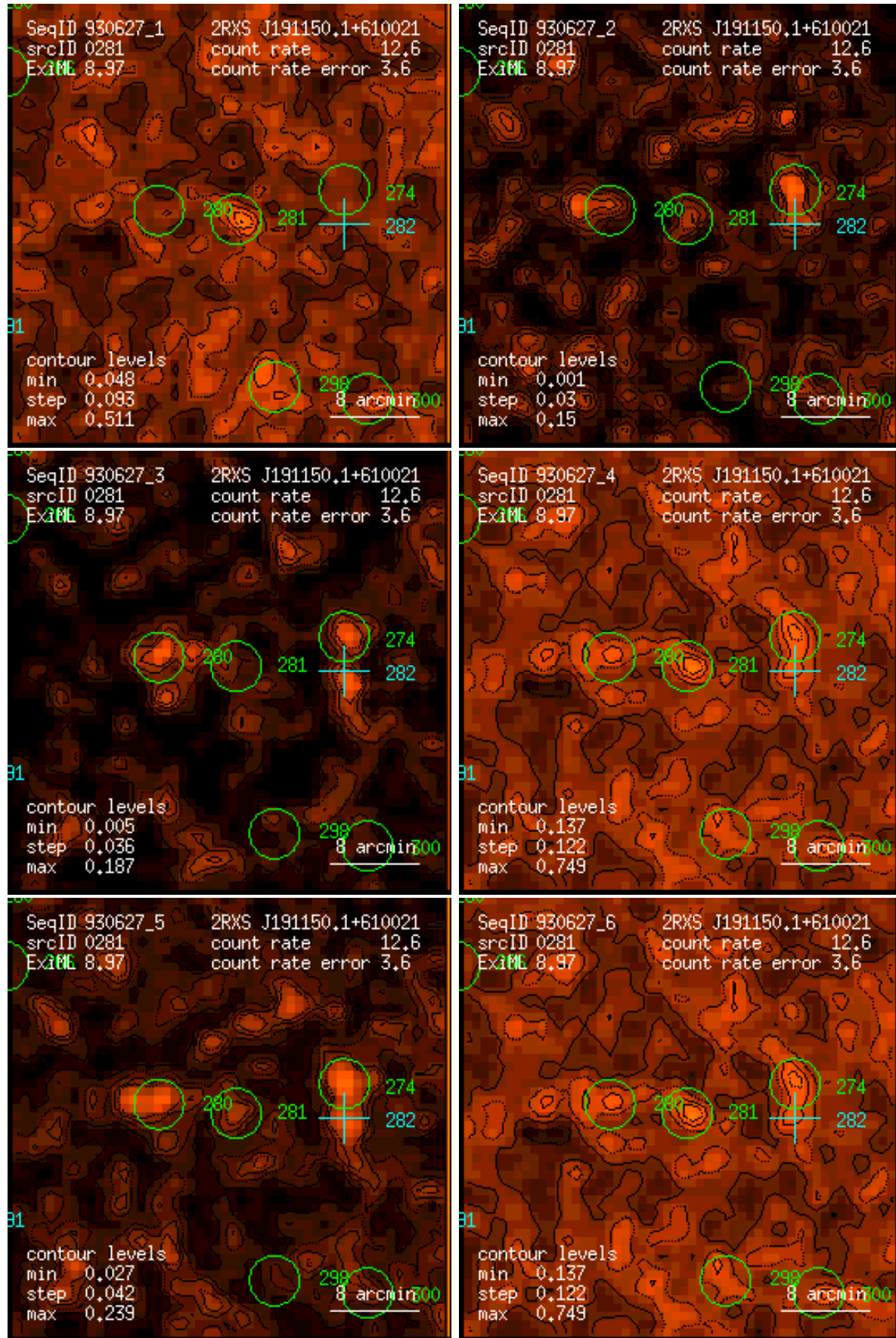
Figure 281: RASS 930627: detection 0281: band rate images, Gaussian filter: (1) PSPC channels 11 – 41, (2) 52 – 90, (3) 91 – 201, (4) 11 – 235, (5) 52 – 201, (6) 11 – 201. Broad band rates in counts/ks. Band rate contour levels in counts/ks/arcmin 2 .
