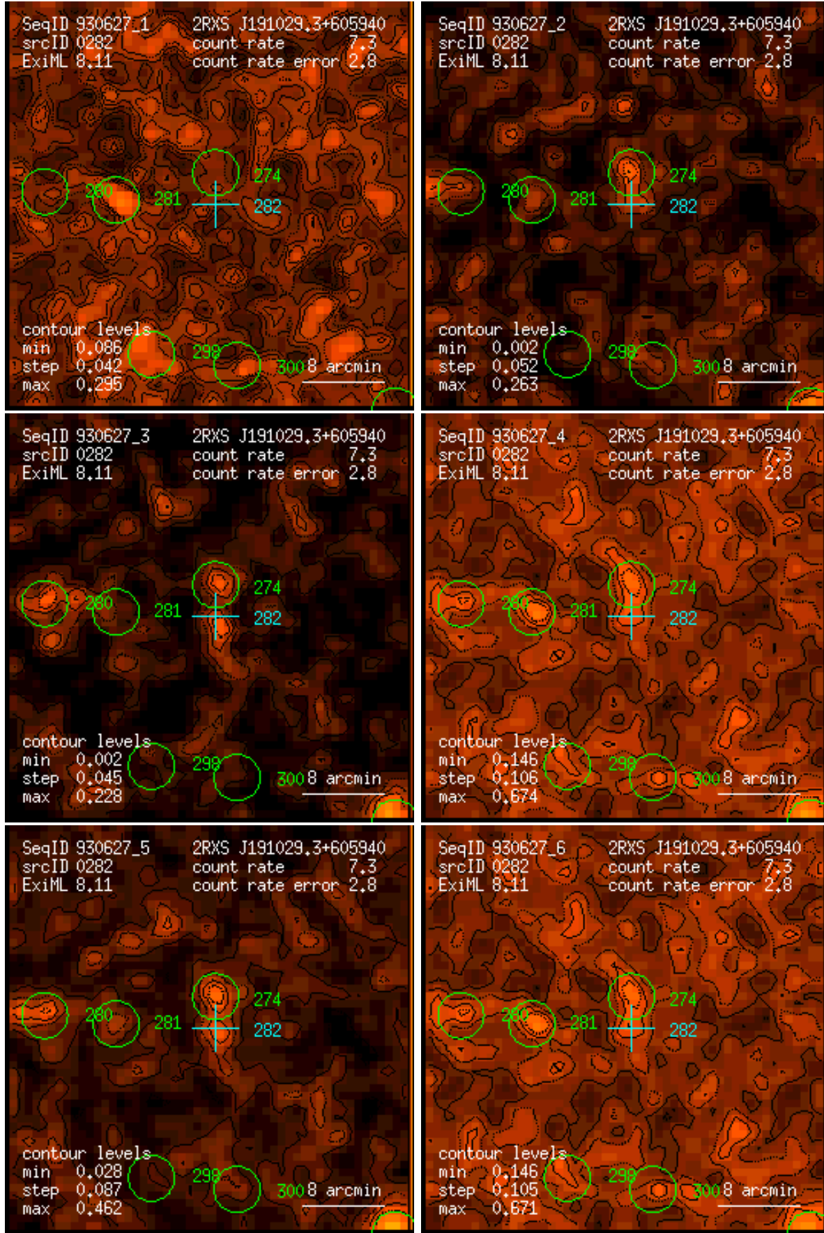
Figure 282: RASS 930627: detection 0282: band rate images, Gaussian filter: (1) PSPC channels 11 – 41, (2) 52 – 90, (3) 91 – 201, (4) 11 – 235, (5) 52 – 201, (6) 11 – 201. Broad band rates in counts/ks. Band rate contour levels in counts/ks/arcmin 2 .
