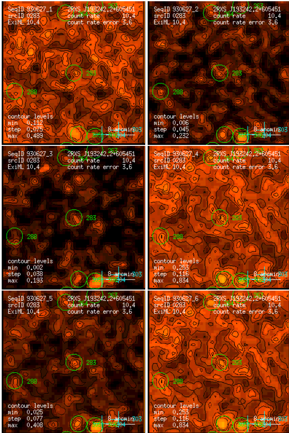
Figure 283: RASS 930627: detection 0283: band rate images, Gaussian filter: (1) PSPC channels 11 – 41, (2) 52 – 90, (3) 91 – 201, (4) 11 – 235, (5) 52 – 201, (6) 11 – 201. Broad band rates in counts/ks. Band rate contour levels in counts/ks/arcmin 2 .
