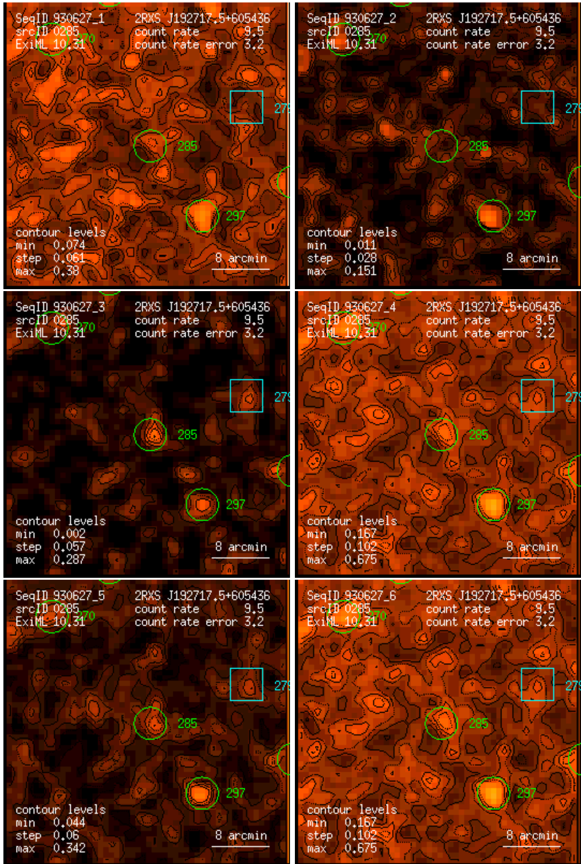
Figure 285: RASS 930627: detection 0285: band rate images, Gaussian filter: (1) PSPC channels 11 – 41, (2) 52 – 90, (3) 91 – 201, (4) 11 – 235, (5) 52 – 201, (6) 11 – 201. Broad band rates in counts/ks. Band rate contour levels in counts/ks/arcmin 2 .
