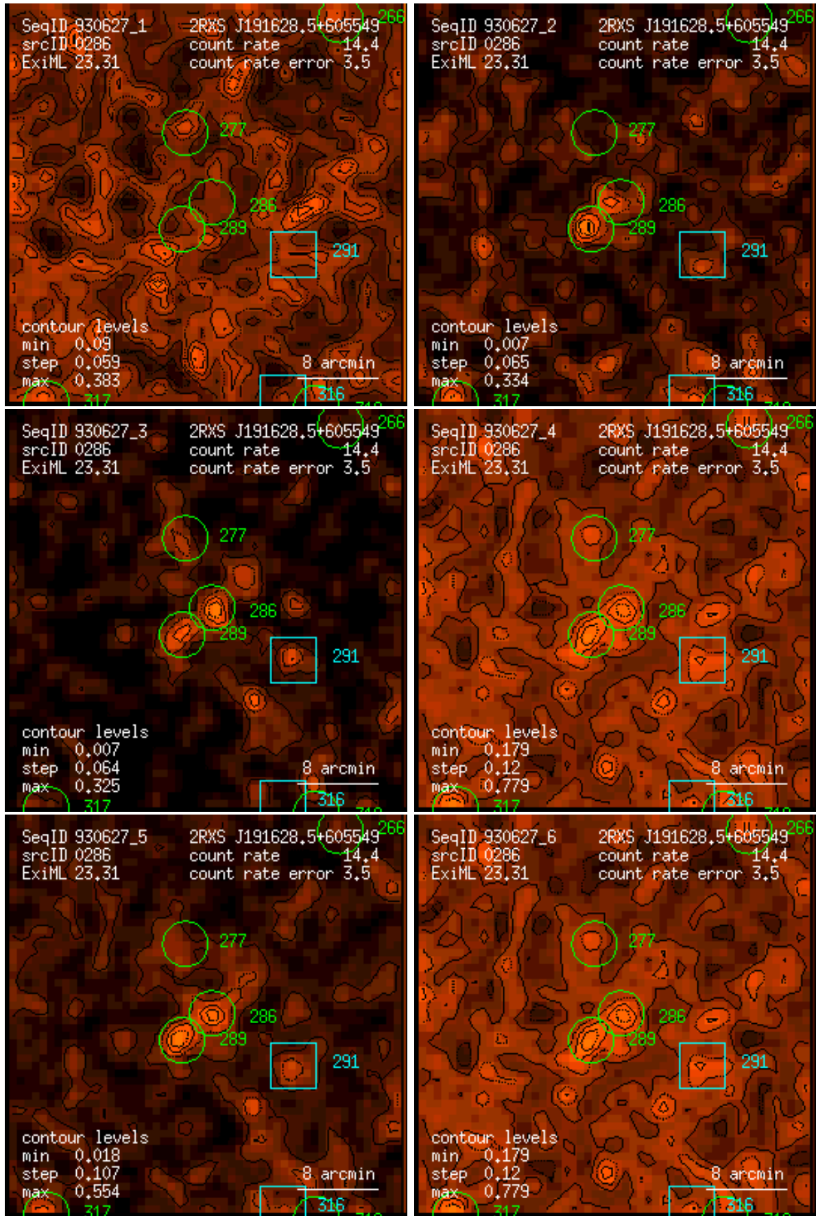
Figure 286: RASS 930627: detection 0286: band rate images, Gaussian filter: (1) PSPPC channels 11 – 41, (2) 52 – 90, (3) 91 – 201, (4) 11 – 235, (5) 52 – 201, (6) 11 – 201. Broad band rates in counts/ks. Band rate contour levels in counts/ks/arcmin 2 .
