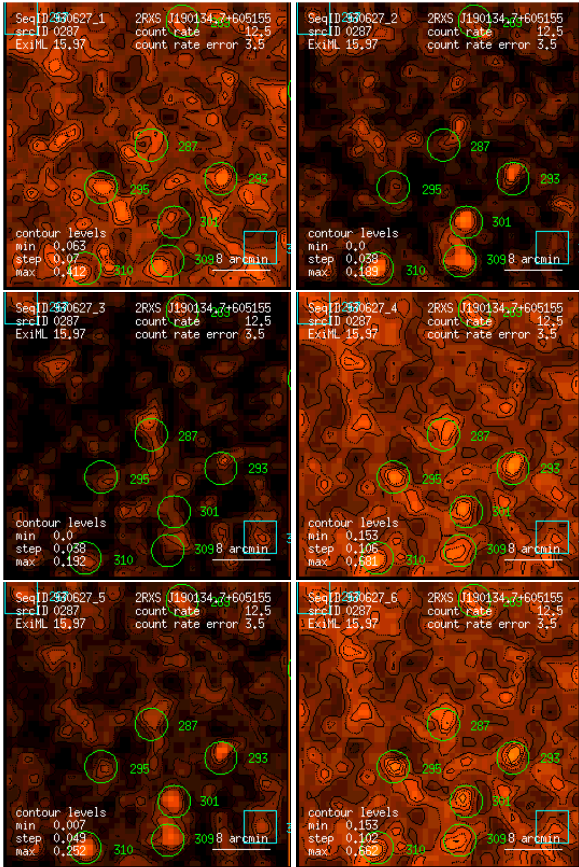
Figure 287: RASS 930627: detection 0287: band rate images, Gaussian filter: (1) PSPC channels 11 – 41, (2) 52 – 90, (3) 91 – 201, (4) 11 – 235, (5) 52 – 201, (6) 11 – 201. Broad band rates in counts/ks. Band rate contour levels in counts/ks/arcmin 2 .
