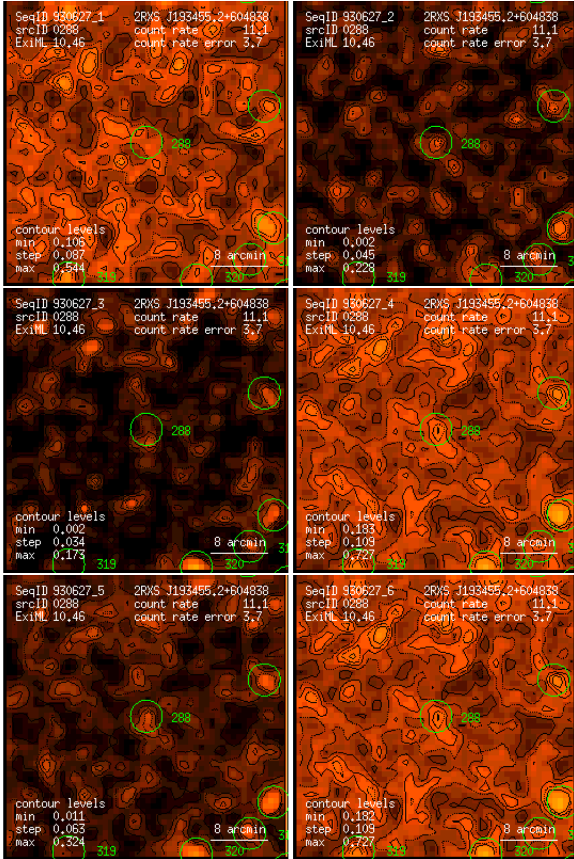
Figure 288: RASS 930627: detection 0288: band rate images, Gaussian filter: (1) PSPC channels 11 – 41, (2) 52 – 90, (3) 91 – 201, (4) 11 – 235, (5) 52 – 201, (6) 11 – 201. Broad band rates in counts/ks. Band rate contour levels in counts/ks/arcmin 2 .
