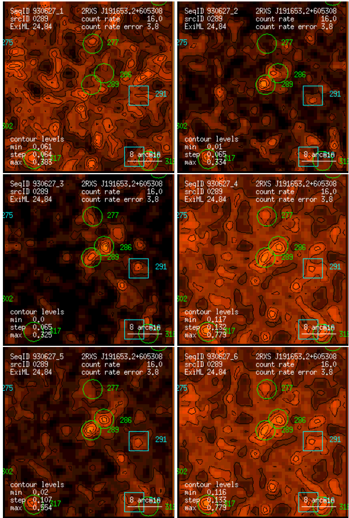
Figure 289: RASS 930627: detection 0289: band rate images, Gaussian filter: (1) PSPC channels 11 – 41, (2) 52 – 90, (3) 91 – 201, (4) 11 – 235, (5) 52 – 201, (6) 11 – 201. Broad band rates in counts/ks. Band rate contour levels in counts/ks/arcmin 2 .
