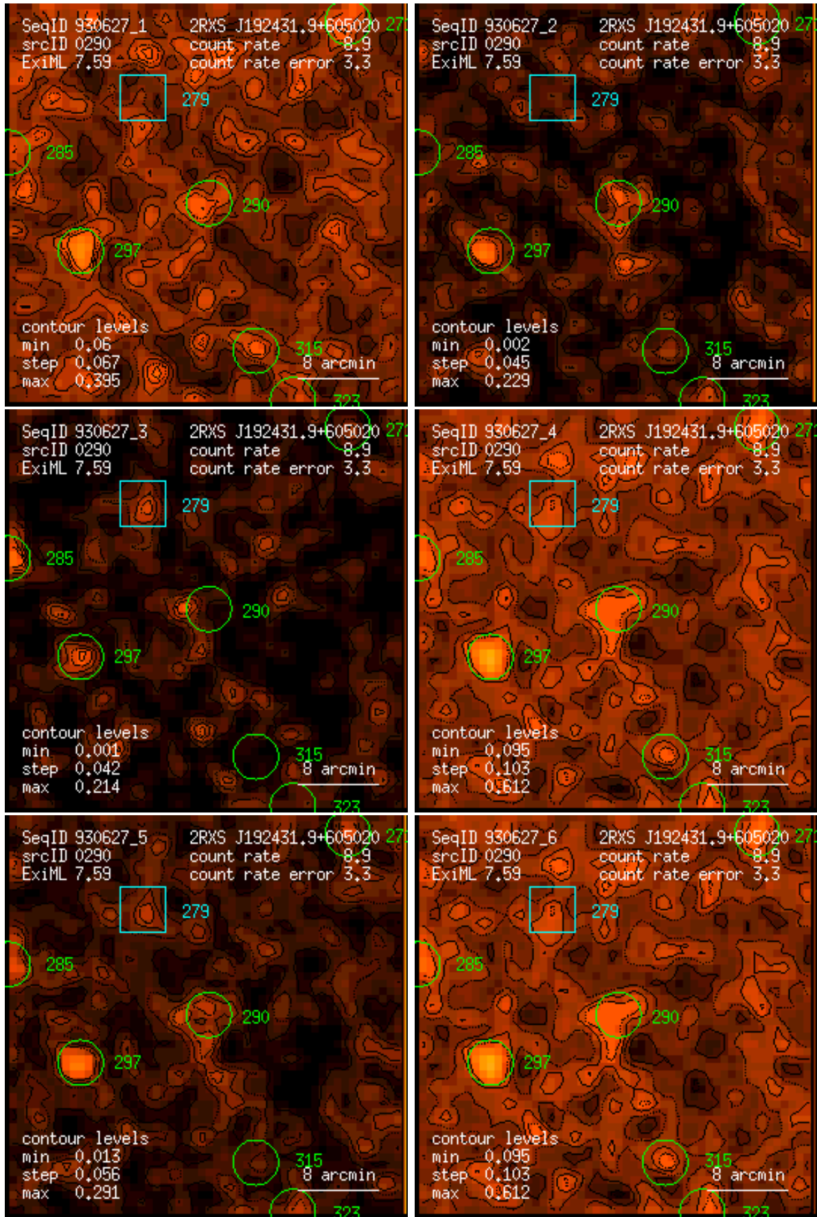
Figure 290: RASS 930627: detection 0290: band rate images, Gaussian filter: (1) PSPC channels 11 – 41, (2) 52 – 90, (3) 91 – 201, (4) 11 – 235, (5) 52 – 201, (6) 11 – 201. Broad band rates in counts/ks. Band rate contour levels in counts/ks/arcmin 2 .
