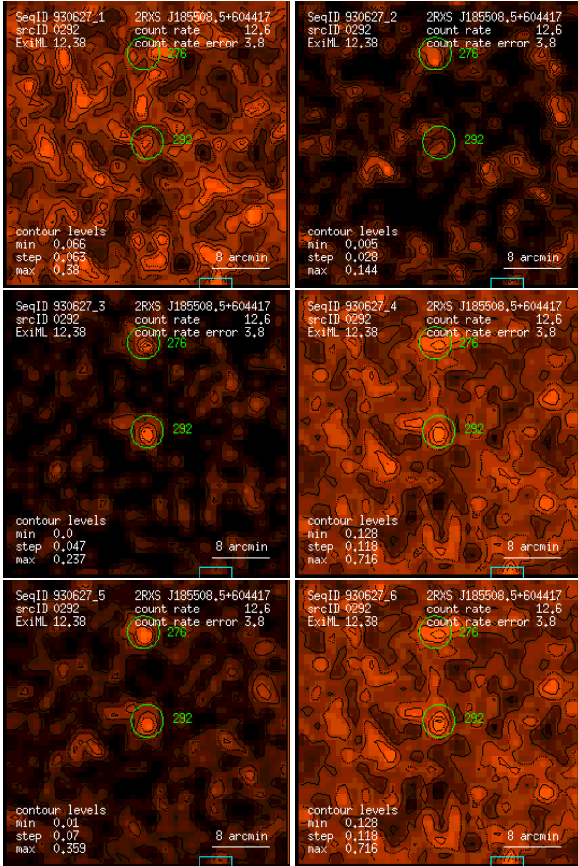
Figure 292: RASS 930627: detection 0292: band rate images, Gaussian filter: (1) PSPC channels 11 – 41, (2) 52 – 90, (3) 91 – 201, (4) 11 – 235, (5) 52 – 201, (6) 11 – 201. Broad band rates in counts/ks. Band rate contour levels in counts/ks/arcmin 2 .
