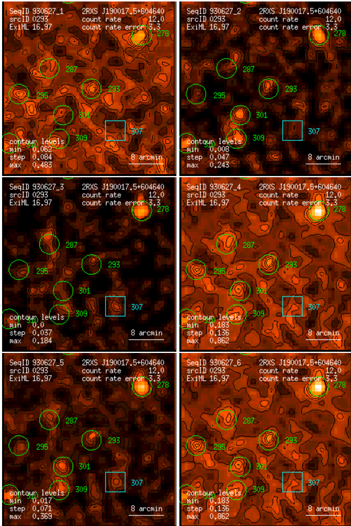
Figure 293: RASS 930627: detection 0293: band rate images, Gaussian filter: (1) PSPC channels 11 – 41, (2) 52 – 90, (3) 91 – 201, (4) 11 – 235, (5) 52 – 201, (6) 11 – 201. Broad band rates in counts/ks. Band rate contour levels in counts/ks/arcmin 2 .
