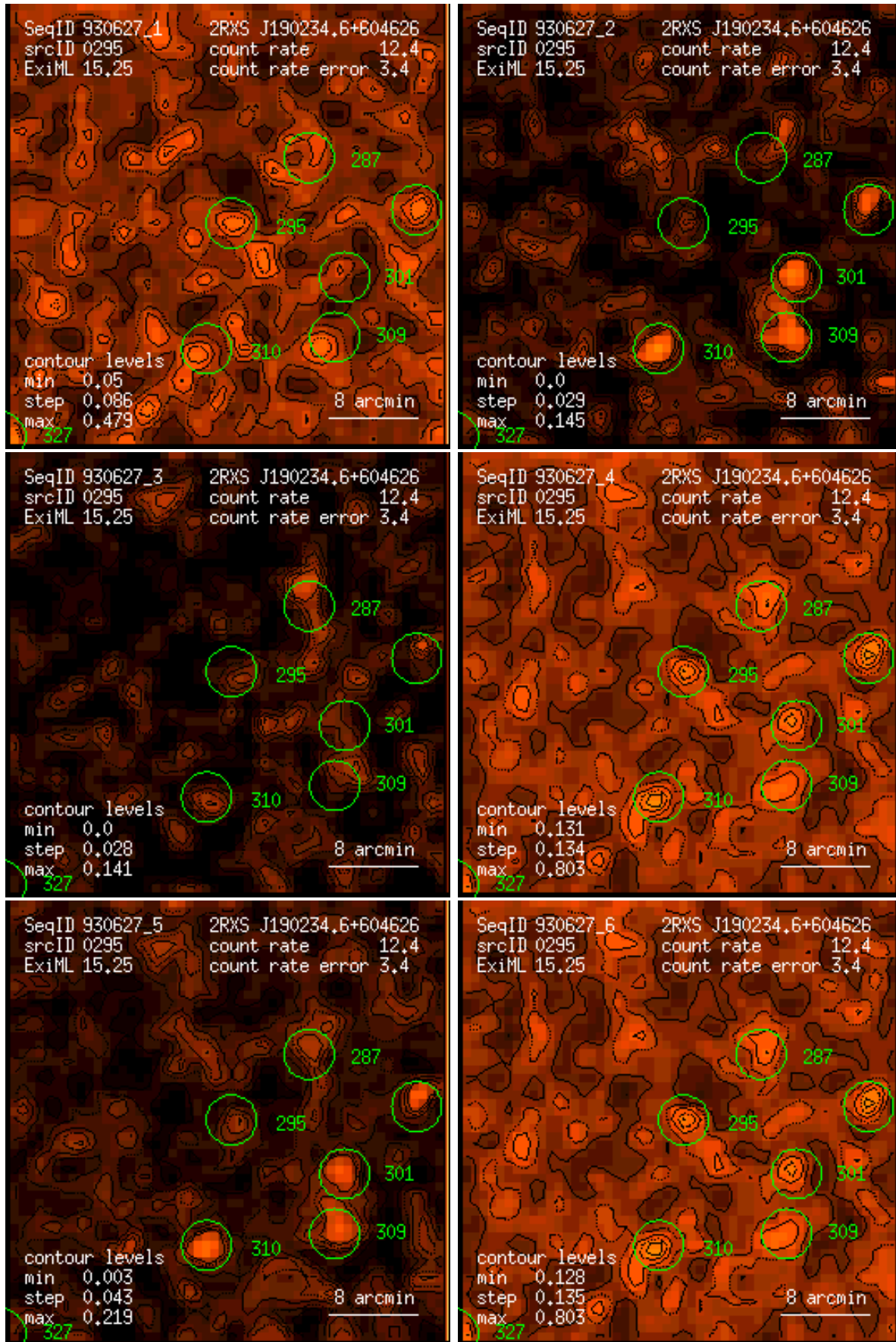
Figure 295: RASS 930627: detection 0295: band rate images, Gaussian filter: (1) PSPC channels 11 – 41, (2) 52 – 90, (3) 91 – 201, (4) 11 – 235, (5) 52 – 201, (6) 11 – 201. Broad band rates in counts/ks. Band rate contour levels in counts/ks/arcmin 2 .
