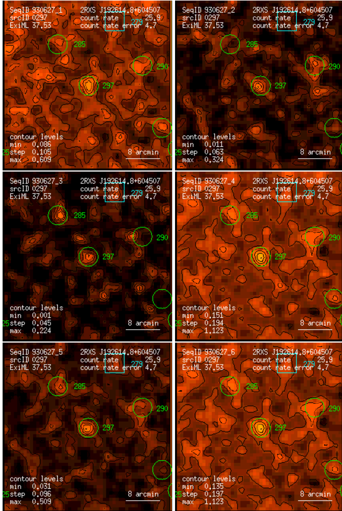
Figure 297: RASS 930627: detection 0297: band rate images, Gaussian filter: (1) PSPC channels 11 – 41, (2) 52 – 90, (3) 91 – 201, (4) 11 – 235, (5) 52 – 201, (6) 11 – 201. Broad band rates in counts/ks. Band rate contour levels in counts/ks/arcmin 2 .
