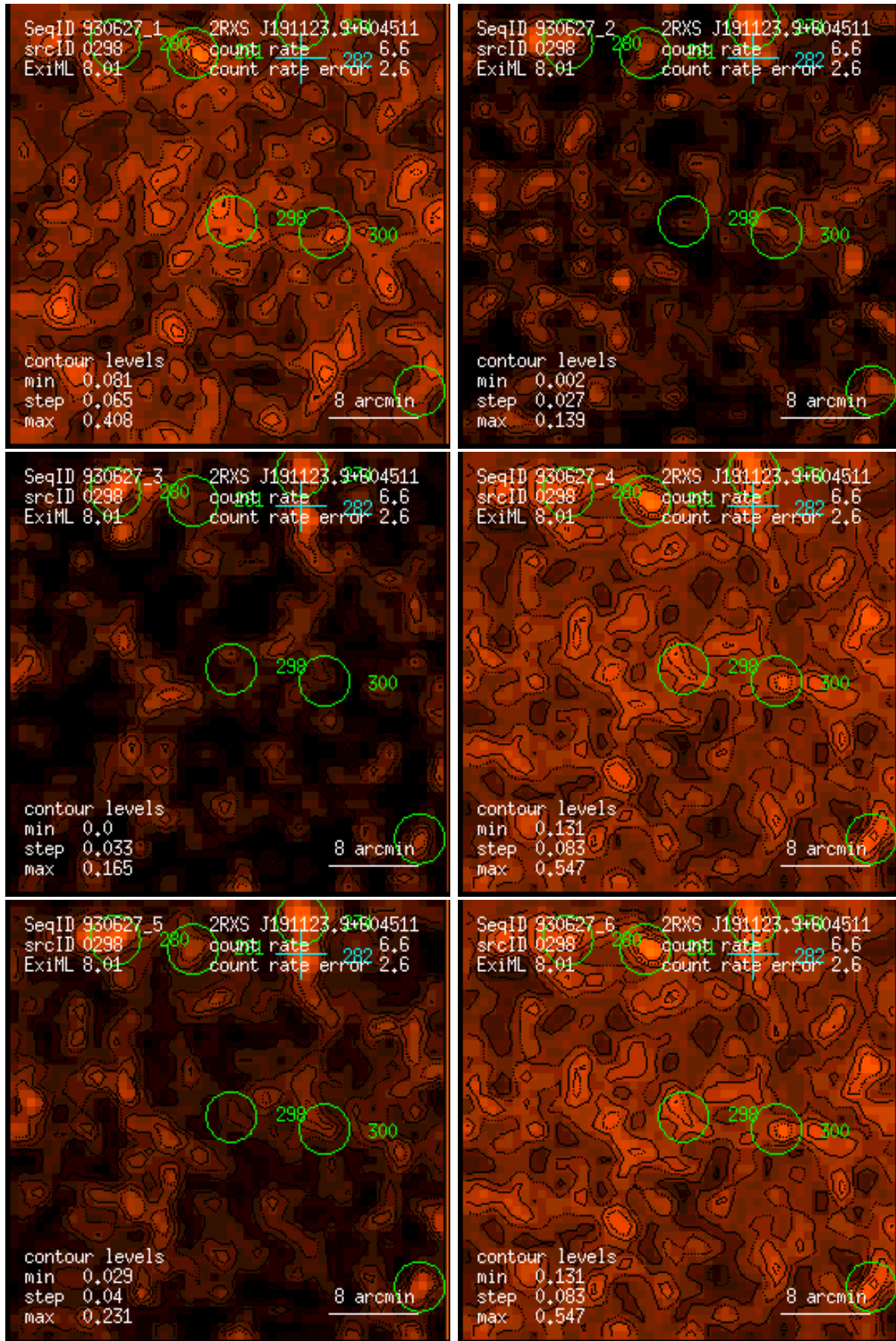
Figure 298: RASS 930627: detection 0298: band rate images, Gaussian filter: (1) PSPC channels 11 – 41, (2) 52 – 90, (3) 91 – 201, (4) 11 – 235, (5) 52 – 201, (6) 11 – 201. Broad band rates in counts/ks. Band rate contour levels in counts/ks/arcmin 2 .
