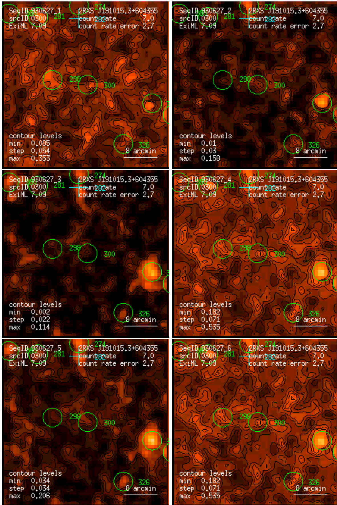
Figure 300: RASS 930627: detection 0300: band rate images, Gaussian filter: (1) PSPC channels 11 – 41, (2) 52 – 90, (3) 91 – 201, (4) 11 – 235, (5) 52 – 201, (6) 11 – 201. Broad band rates in counts/ks. Band rate contour levels in counts/ks/arcmin 2 .
