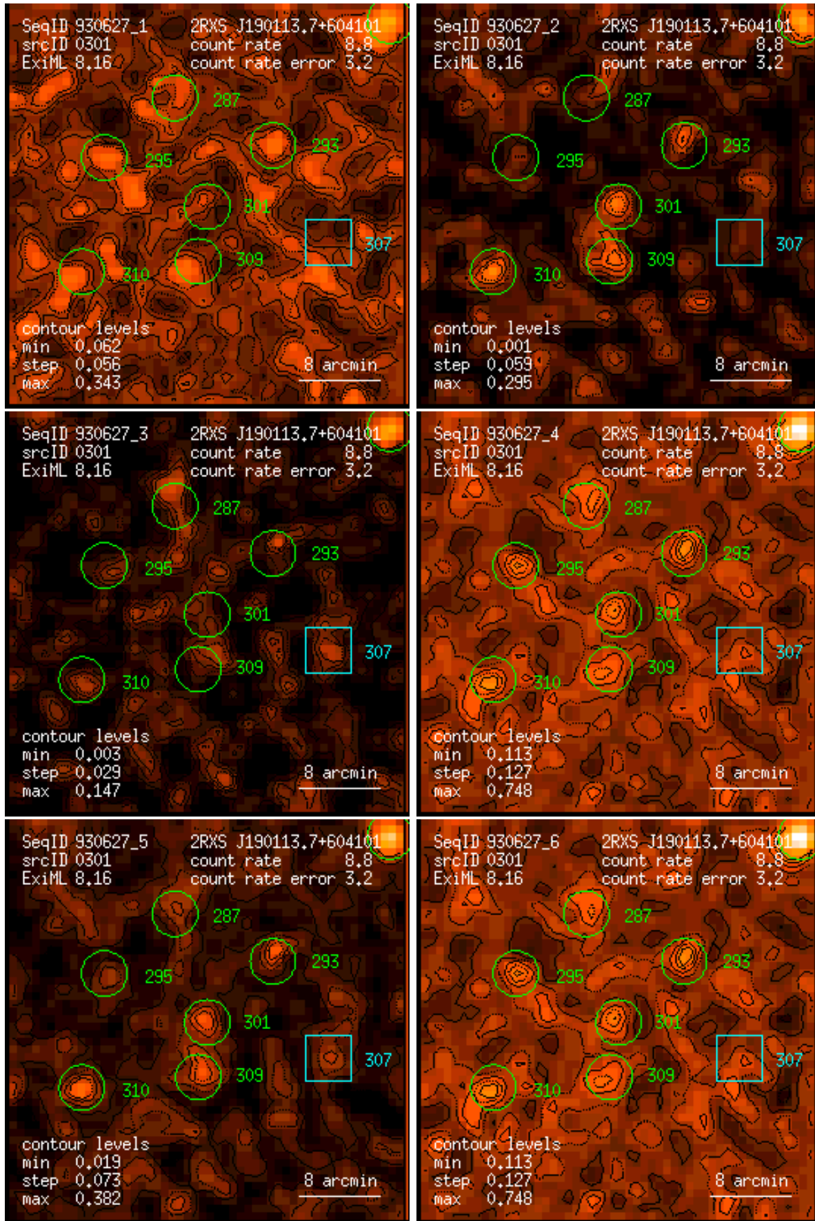
Figure 301: RASS 930627: detection 0301: band rate images, Gaussian filter: (1) PSPC channels 11 – 41, (2) 52 – 90, (3) 91 – 201, (4) 11 – 235, (5) 52 – 201, (6) 11 – 201. Broad band rates in counts/ks. Band rate contour levels in counts/ks/arcmin 2 .
