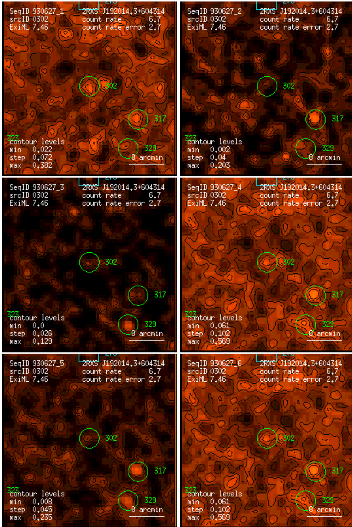
Figure 302: RASS 930627: detection 0302: band rate images, Gaussian filter: (1) PSPC channels 11 – 41, (2) 52 – 90, (3) 91 – 201, (4) 11 – 235, (5) 52 – 201, (6) 11 – 201. Broad band rates in counts/ks. Band rate contour levels in counts/ks/arcmin 2 .
