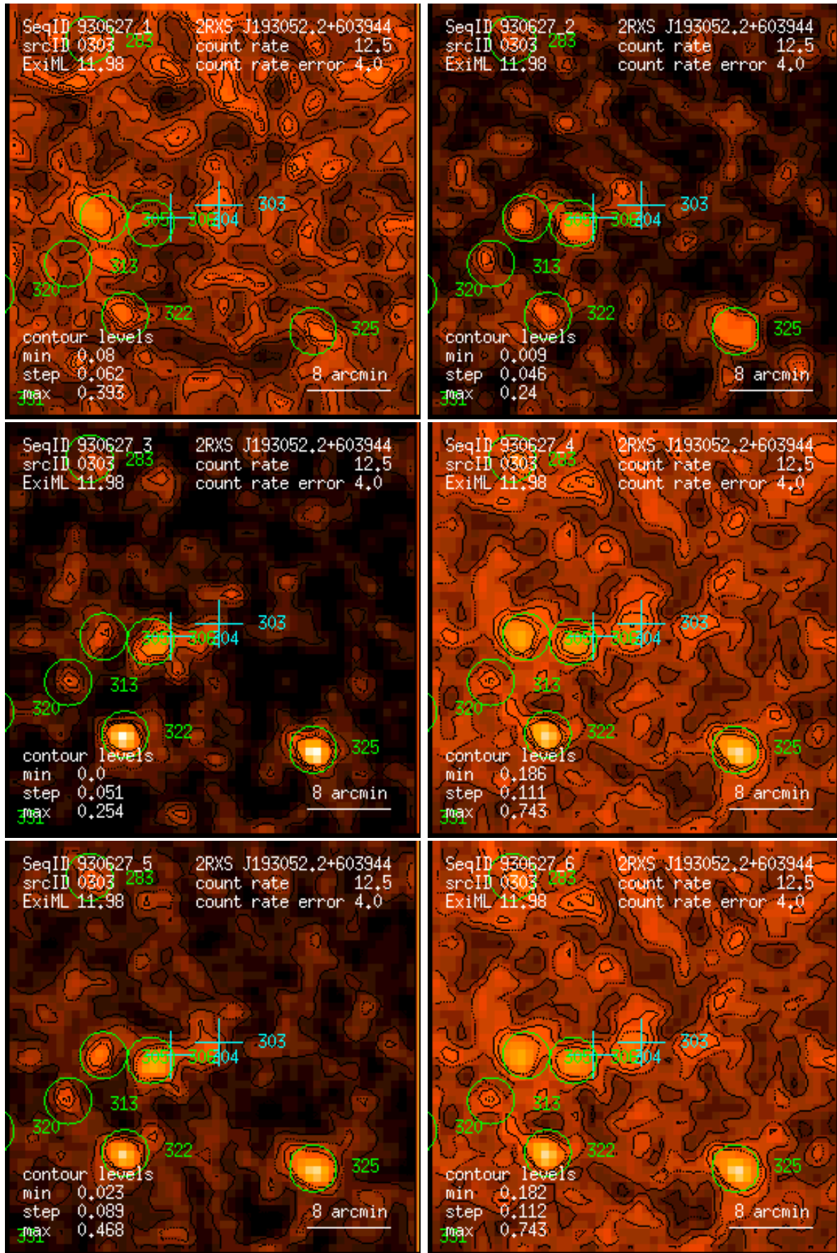
Figure 303: RASS 930627: detection 0303: band rate images, Gaussian filter: (1) PSPC channels 11 – 41, (2) 52 – 90, (3) 91 – 201, (4) 11 – 235, (5) 52 – 201, (6) 11 – 201. Broad band rates in counts/ks. Band rate contour levels in counts/ks/arcmin 2 .
