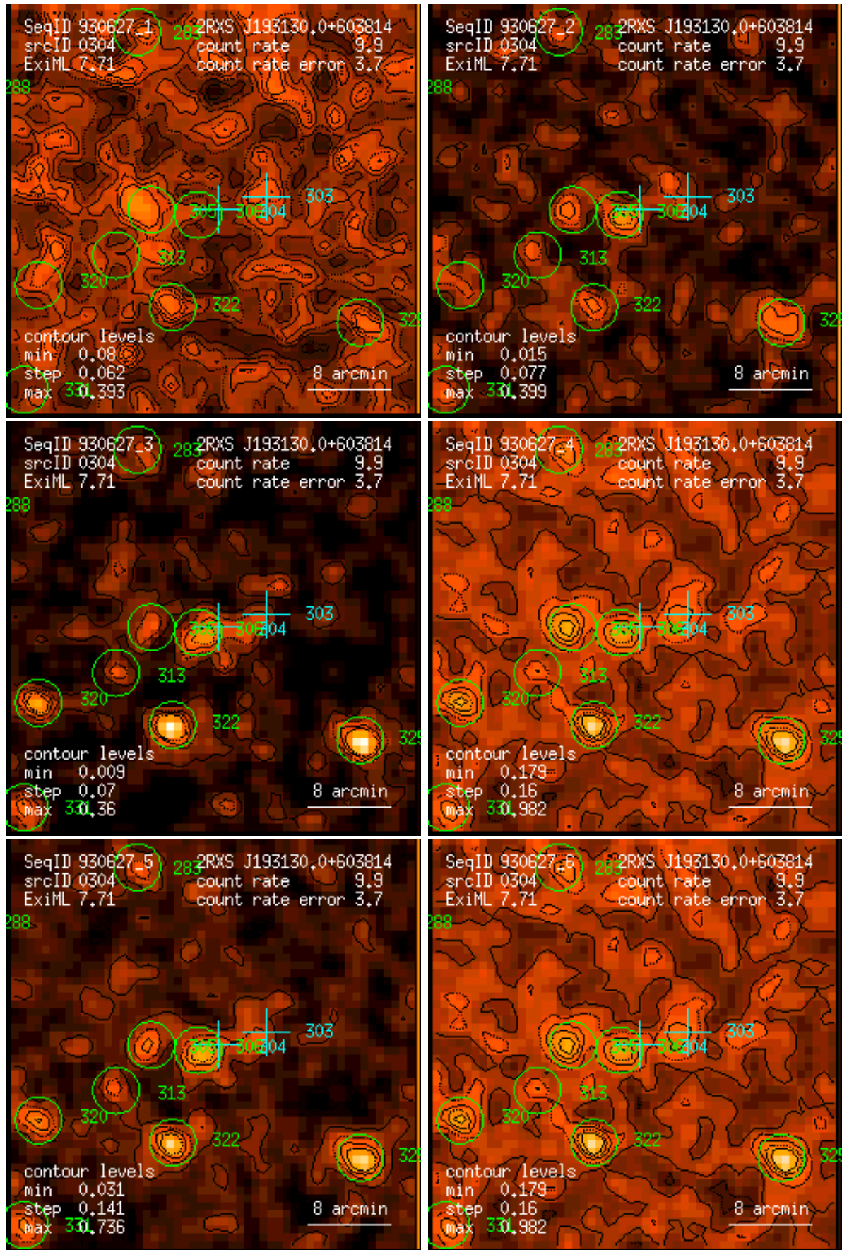
Figure 304: RASS 930627: detection 0304: band rate images, Gaussian filter: (1) PSPC channels 11 – 41, (2) 52 – 90, (3) 91 – 201, (4) 11 – 235, (5) 52 – 201, (6) 11 – 201. Broad band rates in counts/ks. Band rate contour levels in counts/ks/arcmin 2 .
