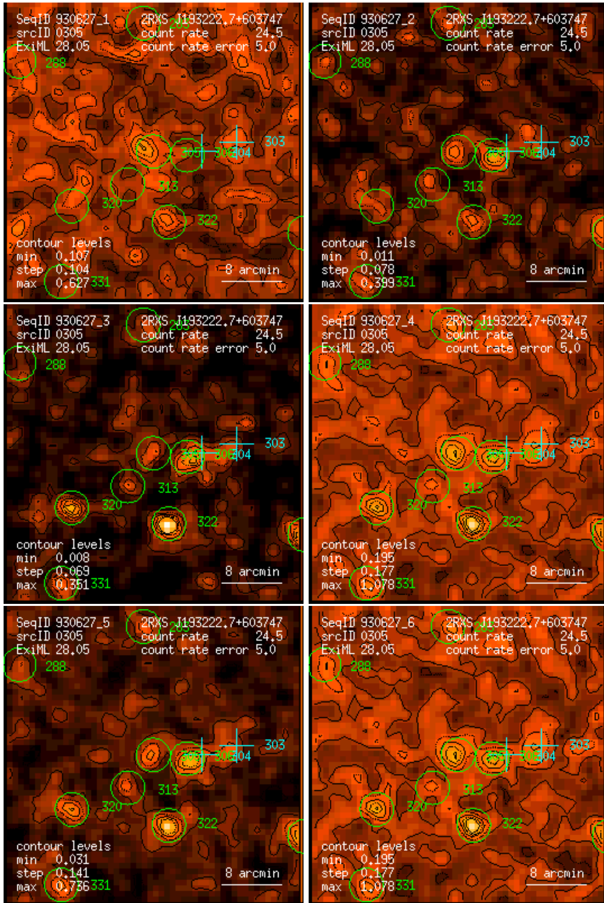
Figure 305: RASS 930627: detection 0305: band rate images, Gaussian filter: (1) PSPC channels 11 – 41, (2) 52 – 90, (3) 91 – 201, (4) 11 – 235, (5) 52 – 201, (6) 11 – 201. Broad band rates in counts/ks. Band rate contour levels in counts/ks/arcmin 2 .
