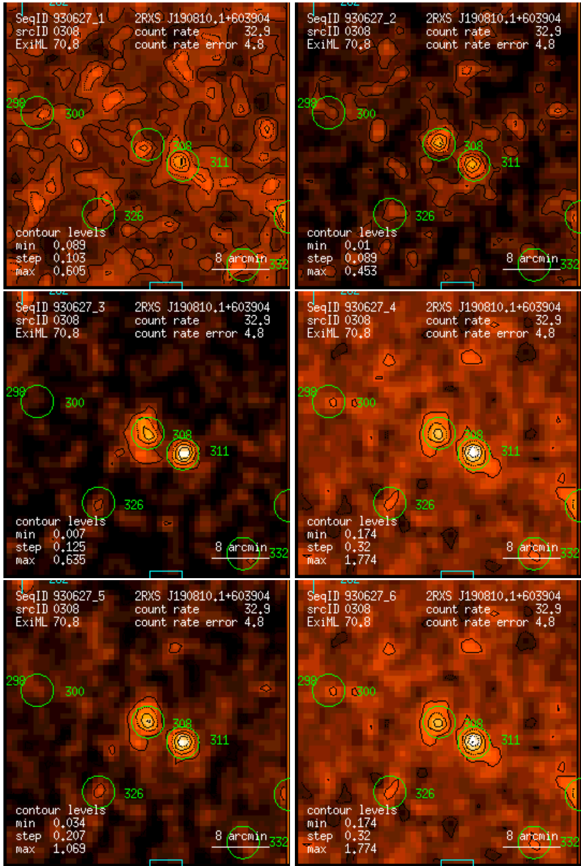
Figure 308: RASS 930627: detection 0308: band rate images, Gaussian filter: (1) PSPC channels 11 – 41, (2) 52 – 90, (3) 91 – 201, (4) 11 – 235, (5) 52 – 201, (6) 11 – 201. Broad band rates in counts/ks. Band rate contour levels in counts/ks/arcmin 2 .
