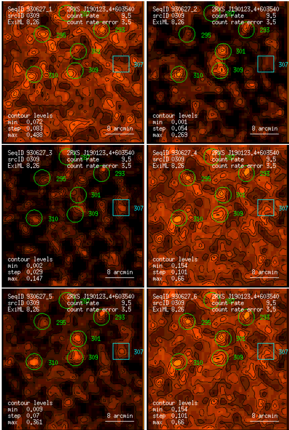
Figure 309: RASS 930627: detection 0309: band rate images, Gaussian filter: (1) PSPC channels 11 – 41, (2) 52 – 90, (3) 91 – 201, (4) 11 – 235, (5) 52 – 201, (6) 11 – 201. Broad band rates in counts/ks. Band rate contour levels in counts/ks/arcmin 2 .
