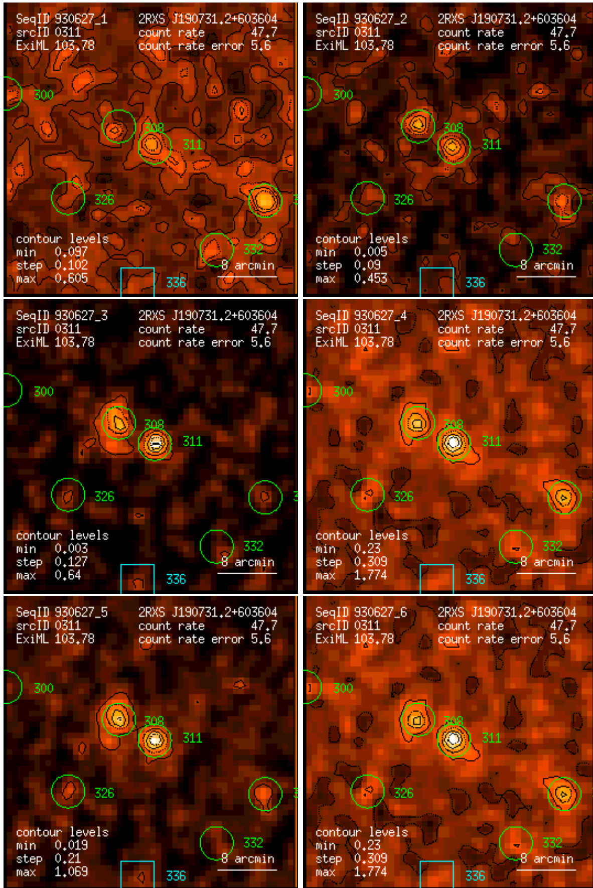
Figure 311: RASS 930627: detection 0311: band rate images, Gaussian filter: (1) PSPC channels 11 – 41, (2) 52 – 90, (3) 91 – 201, (4) 11 – 235, (5) 52 – 201, (6) 11 – 201. Broad band rates in counts/ks. Band rate contour levels in counts/ks/arcmin 2 .
