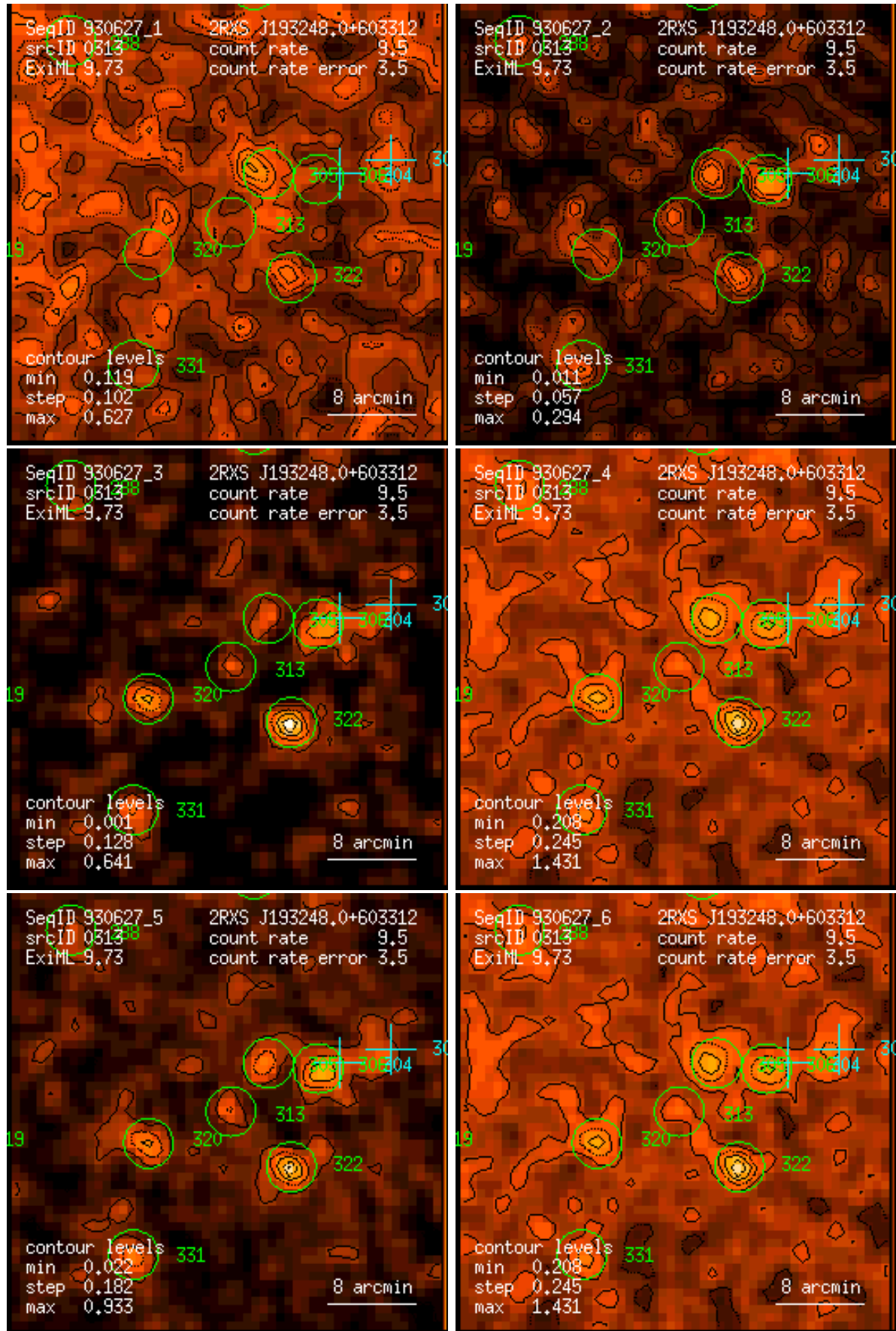
Figure 313: RASS 930627: detection 0313: band rate images, Gaussian filter: (1) PSPC channels 11 – 41, (2) 52 – 90, (3) 91 – 201, (4) 11 – 235, (5) 52 – 201, (6) 11 – 201. Broad band rates in counts/ks. Band rate contour levels in counts/ks/arcmin 2 .
