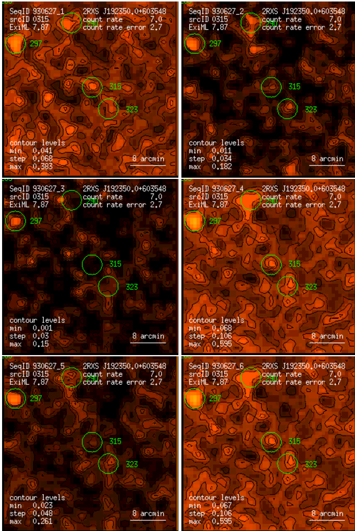
Figure 315: RASS 930627: detection 0315: band rate images, Gaussian filter: (1) PSPC channels 11 – 41, (2) 52 – 90, (3) 91 – 201, (4) 11 – 235, (5) 52 – 201, (6) 11 – 201. Broad band rates in counts/ks. Band rate contour levels in counts/ks/arcmin 2 .
