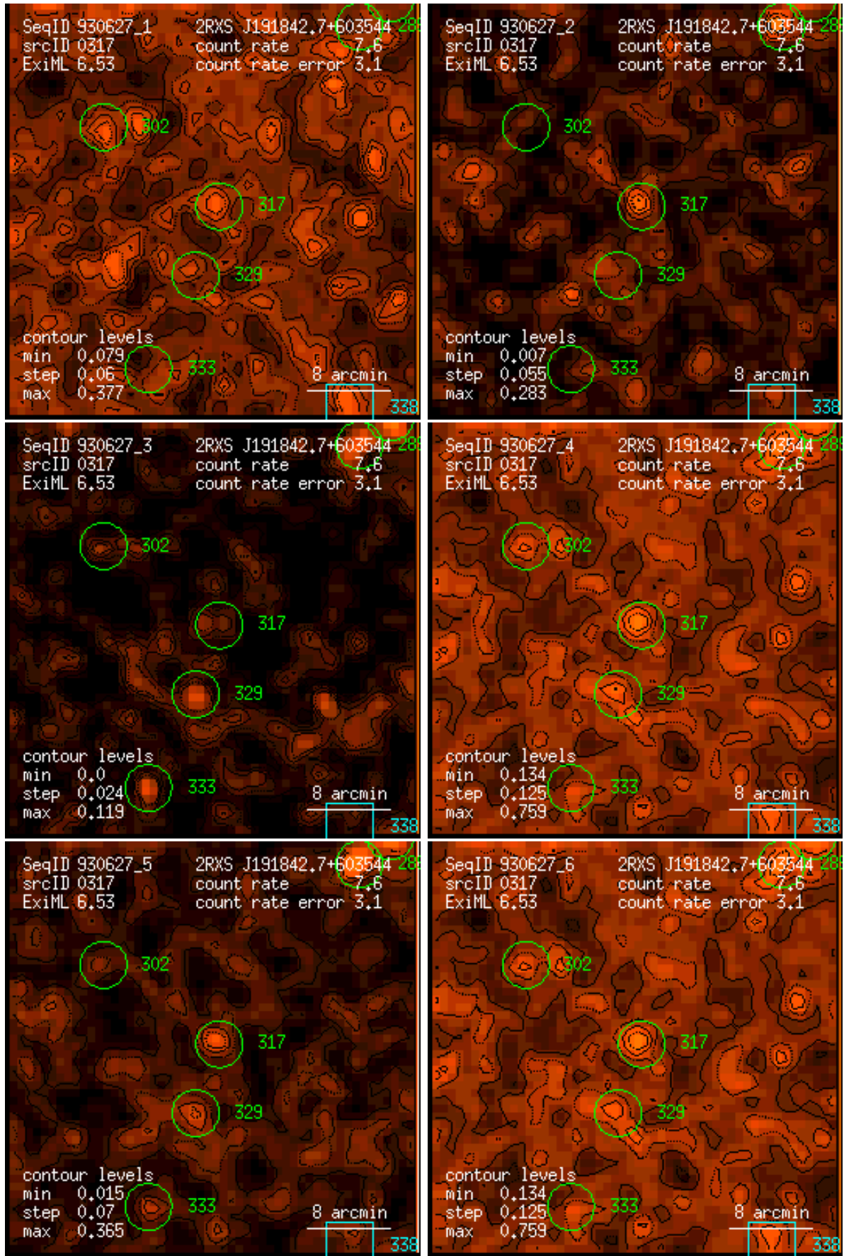
Figure 317: RASS 930627: detection 0317: band rate images, Gaussian filter: (1) PSPC channels 11 – 41, (2) 52 – 90, (3) 91 – 201, (4) 11 – 235, (5) 52 – 201, (6) 11 – 201. Broad band rates in counts/ks. Band rate contour levels in counts/ks/arcmin 2 .
