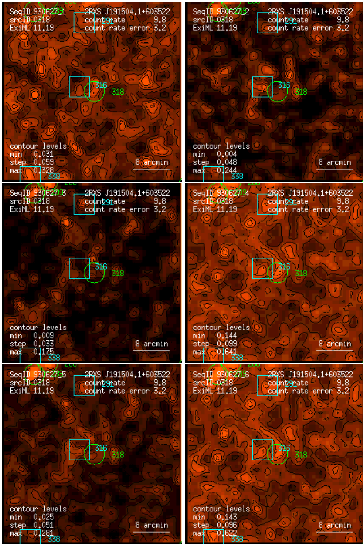
Figure 318: RASS 930627: detection 0318: band rate images, Gaussian filter: (1) PSPC channels 11 – 41, (2) 52 – 90, (3) 91 – 201, (4) 11 – 235, (5) 52 – 201, (6) 11 – 201. Broad band rates in counts/ks. Band rate contour levels in counts/ks/arcmin 2 .
