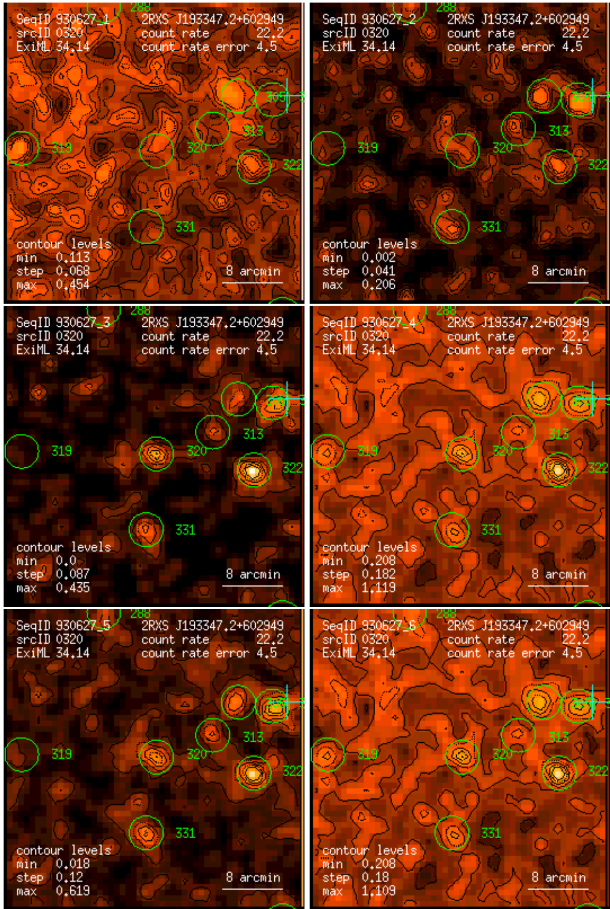
Figure 320: RASS 930627: detection 0320: band rate images, Gaussian filter: (1) PSPC channels 11 – 41, (2) 52 – 90, (3) 91 – 201, (4) 11 – 235, (5) 52 – 201, (6) 11 – 201. Broad band rates in counts/ks. Band rate contour levels in counts/ks/arcmin 2 .
