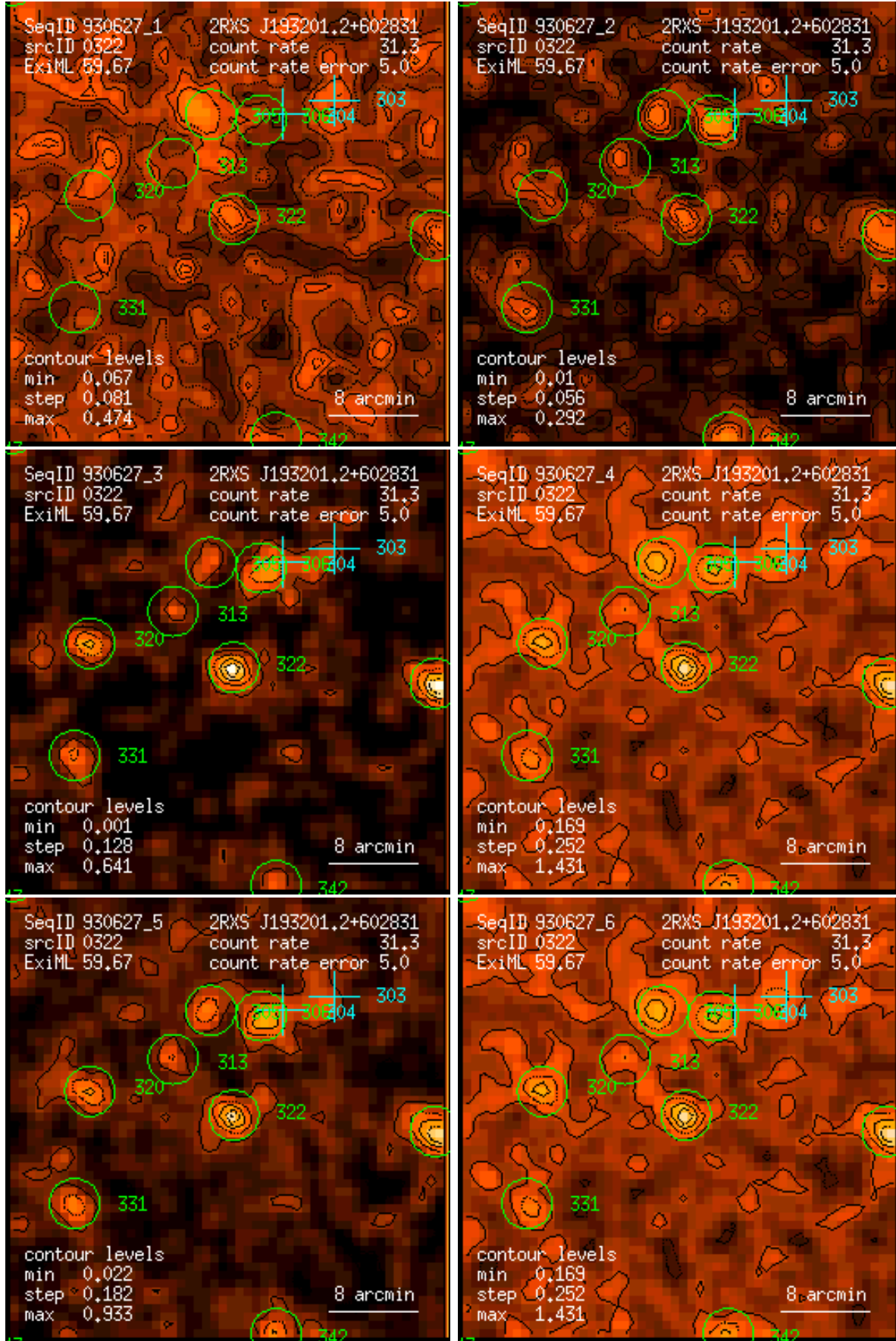
Figure 322: RASS 930627: detection 0322: band rate images, Gaussian filter: (1) PSPC channels 11 – 41, (2) 52 – 90, (3) 91 – 201, (4) 11 – 235, (5) 52 – 201, (6) 11 – 201. Broad band rates in counts/ks. Band rate contour levels in counts/ks/arcmin 2 .
