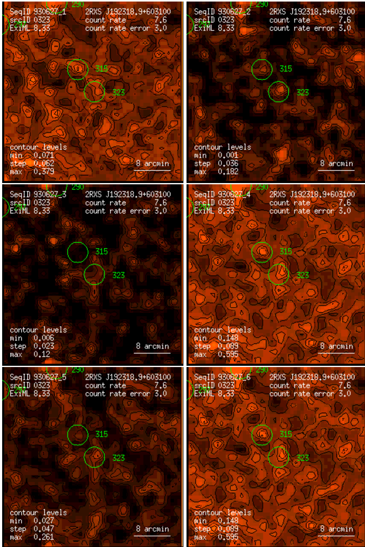
Figure 323: RASS 930627: detection 0323: band rate images, Gaussian filter: (1) PSPC channels 11 – 41, (2) 52 – 90, (3) 91 – 201, (4) 11 – 235, (5) 52 – 201, (6) 11 – 201. Broad band rates in counts/ks. Band rate contour levels in counts/ks/arcmin 2 .
