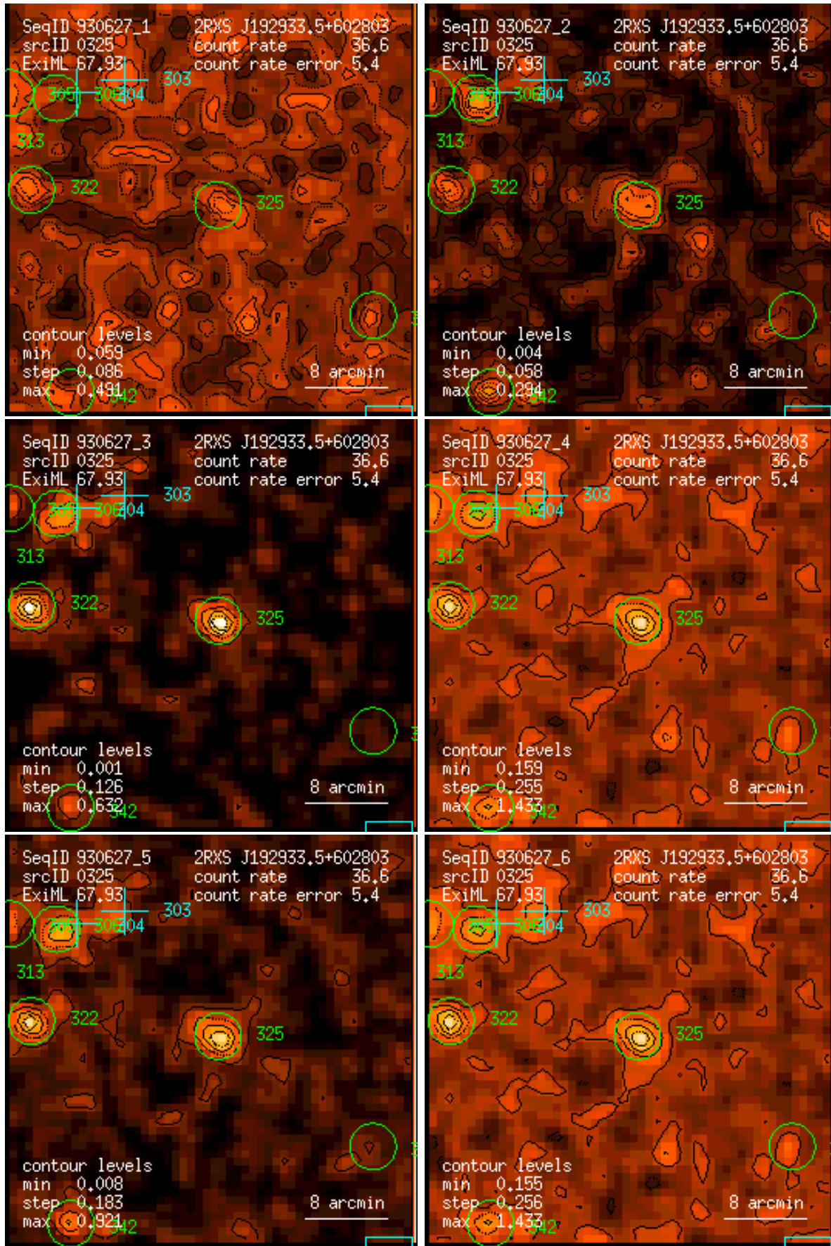
Figure 325: RASS 930627: detection 0325: band rate images, Gaussian filter: (1) PSPC channels 11 – 41, (2) 52 – 90, (3) 91 – 201, (4) 11 – 235, (5) 52 – 201, (6) 11 – 201. Broad band rates in counts/ks. Band rate contour levels in counts/ks/arcmin 2 .
