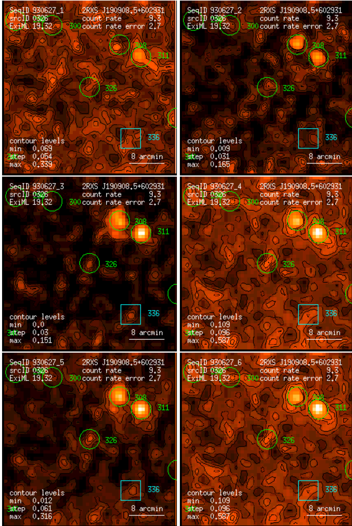
Figure 326: RASS 930627: detection 0326: band rate images, Gaussian filter: (1) PSPC channels 11 – 41, (2) 52 – 90, (3) 91 – 201, (4) 11 – 235, (5) 52 – 201, (6) 11 – 201. Broad band rates in counts/ks. Band rate contour levels in counts/ks/arcmin 2 .
