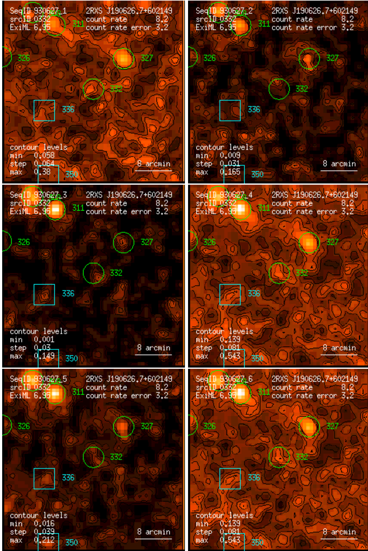
Figure 332: RASS 930627: detection 0332: band rate images, Gaussian filter: (1) PSPC channels 11 – 41, (2) 52 – 90, (3) 91 – 201, (4) 11 – 235, (5) 52 – 201, (6) 11 – 201. Broad band rates in counts/ks. Band rate contour levels in counts/ks/arcmin 2 .
