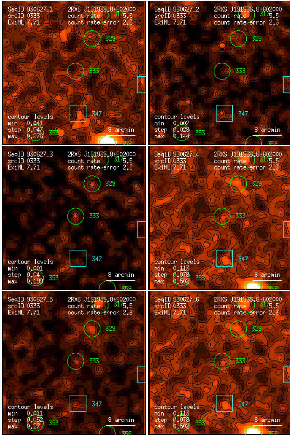
Figure 333: RASS 930627: detection 0333: band rate images, Gaussian filter: (1) PSPC channels 11 – 41, (2) 52 – 90, (3) 91 – 201, (4) 11 – 235, (5) 52 – 201, (6) 11 – 201. Broad band rates in counts/ks. Band rate contour levels in counts/ks/arcmin 2 .
