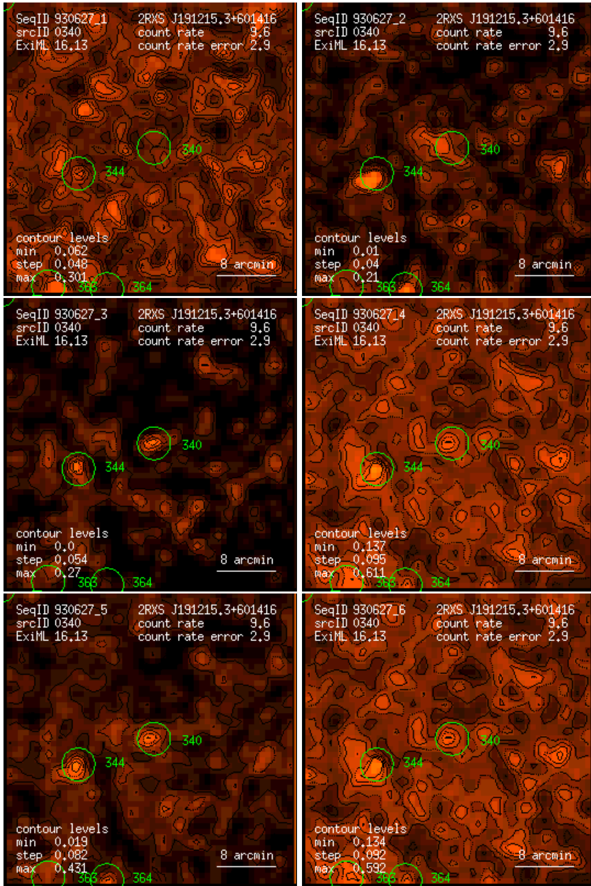
Figure 340: RASS 930627: detection 0340: band rate images, Gaussian filter: (1) PSPC channels 11 – 41, (2) 52 – 90, (3) 91 – 201, (4) 11 – 235, (5) 52 – 201, (6) 11 – 201. Broad band rates in counts/ks. Band rate contour levels in counts/ks/arcmin 2 .
