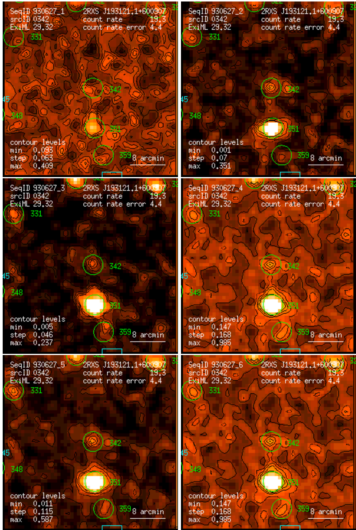
Figure 342: RASS 930627: detection 0342: band rate images, Gaussian filter: (1) PSPC channels 11 – 41, (2) 52 – 90, (3) 91 – 201, (4) 11 – 235, (5) 52 – 201, (6) 11 – 201. Broad band rates in counts/ks. Band rate contour levels in counts/ks/arcmin 2 .
