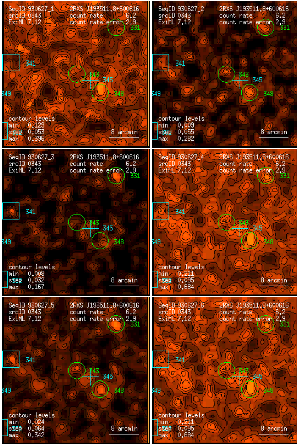
Figure 343: RASS 930627: detection 0343: band rate images, Gaussian filter: (1) PSPC channels 11 – 41, (2) 52 – 90, (3) 91 – 201, (4) 11 – 235, (5) 52 – 201, (6) 11 – 201. Broad band rates in counts/ks. Band rate contour levels in counts/ks/arcmin 2 .
