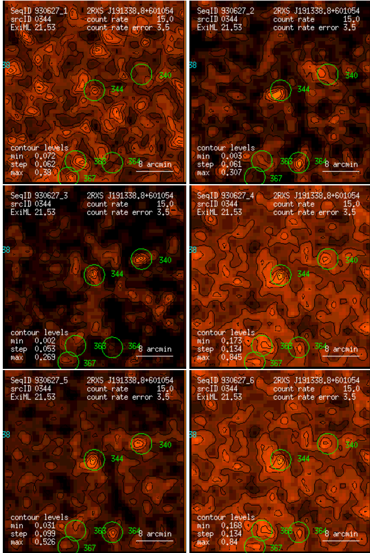
Figure 344: RASS 930627: detection 0344: band rate images, Gaussian filter: (1) PSPC channels 11 – 41, (2) 52 – 90, (3) 91 – 201, (4) 11 – 235, (5) 52 – 201, (6) 11 – 201. Broad band rates in counts/ks. Band rate contour levels in counts/ks/arcmin 2 .
