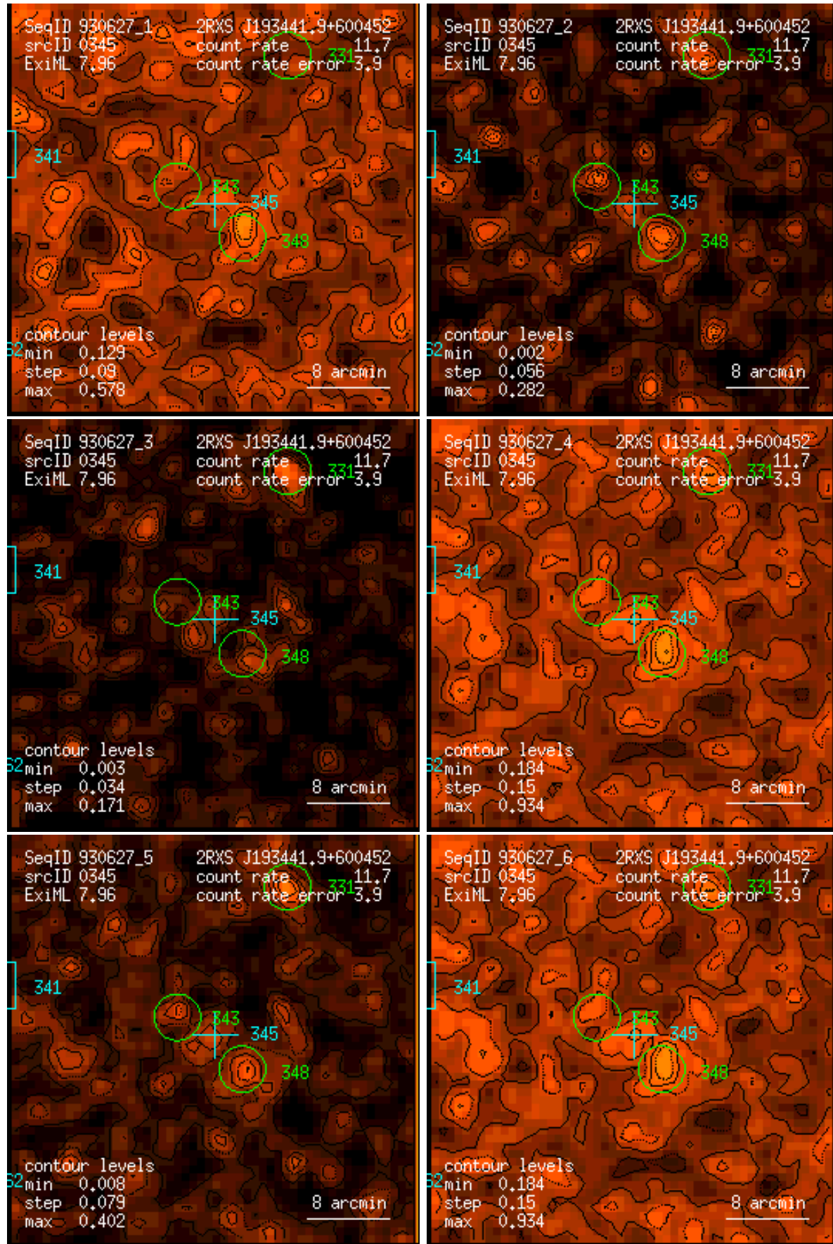
Figure 345: RASS 930627: detection 0345: band rate images, Gaussian filter: (1) PSPC channels 11 – 41, (2) 52 – 90, (3) 91 – 201, (4) 11 – 235, (5) 52 – 201, (6) 11 – 201. Broad band rates in counts/ks. Band rate contour levels in counts/ks/arcmin 2 .
