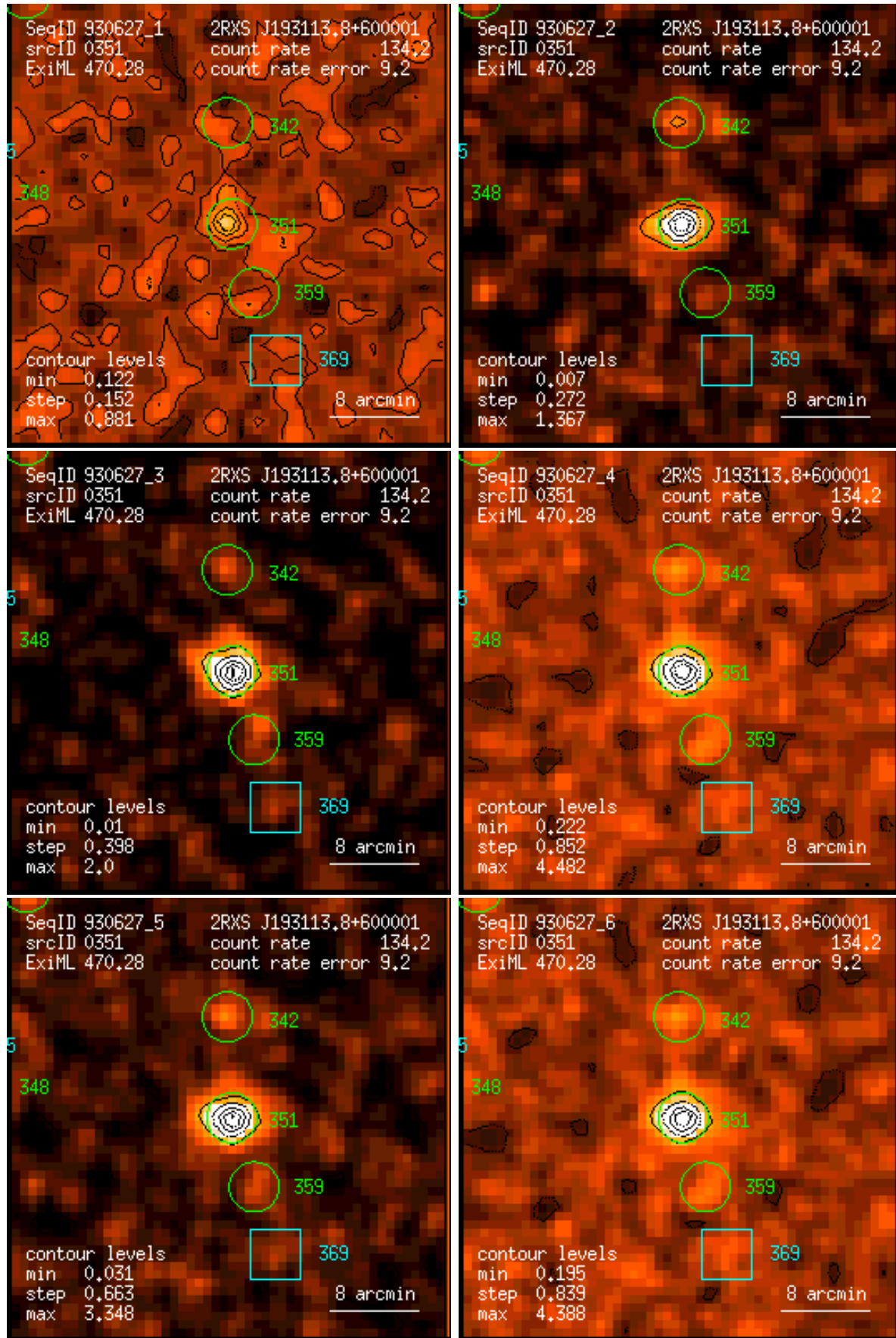
Figure 351: RASS 930627: detection 0351: band rate images, Gaussian filter: (1) PSPC channels 11 – 41, (2) 52 – 90, (3) 91 – 201, (4) 11 – 235, (5) 52 – 201, (6) 11 – 201. Broad band rates in counts/ks. Band rate contour levels in counts/ks/arcmin 2 .
